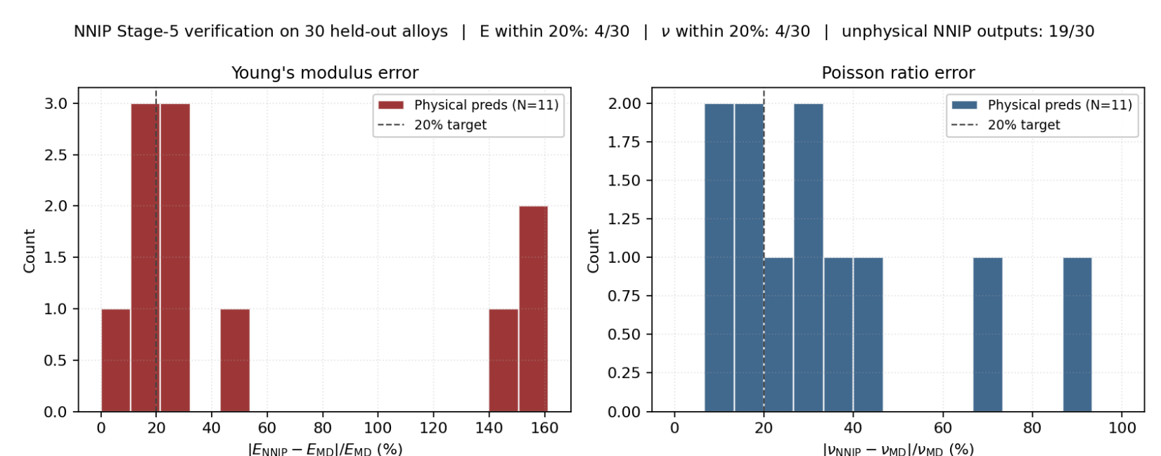
Figure 6. Verification of the optimized potential against the MD reference on unseen alloys.
