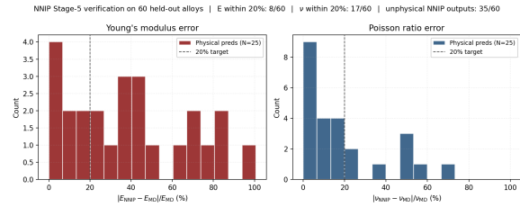
Figure 13: Verification error over the 25 physical predictions among the 60 held-out alloys, for E (left) and \nu (right); the dashed line marks the 20 % tolerance. Eight of the 25 land within tolerance on E and 17 on \nu ; the 35 alloys with unphysical outputs are excluded from the histograms.
