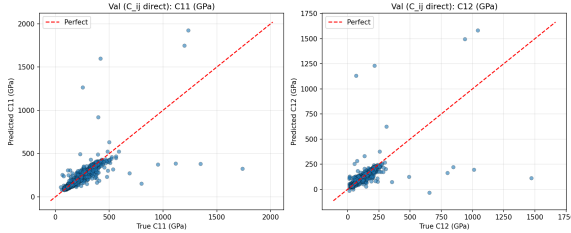
Figure 8: Held-out parity on the raw targets C_{11} and C_{12} , the quantities the network actually regresses.
