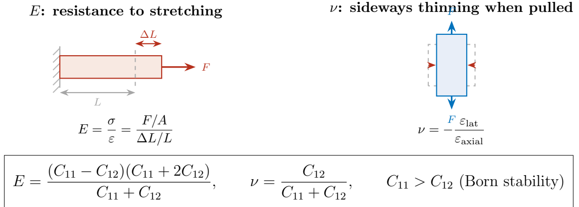
Figure 1: The two elastic moduli this work predicts. Left : a uniaxial force F stretches a bar by \Delta L , and the stiffness E = \sigma/\varepsilon is the stress-to-strain ratio. Right : the same axial pull makes the block contract laterally, and \nu is the negated ratio of lateral to axial strain. For a cubic crystal both reduce to the two independent stiffness constants C_{11} and C_{12} (boxed), and mechanical stability requires C_{11} > C_{12} .
