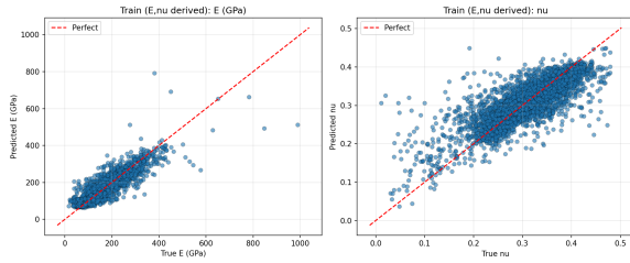
Figure 7: Training-set parity for the predicted E and \nu .
