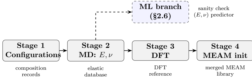
Figure 1: Four-stage pipeline architecture (solid arrows) plus the divergent ML sanity-check branch (dashed) described in Section 2.6. Each main stage is implemented as an independent Python module and communicates with the next one through JSON or MEAM-format files written to disk; the ML branch consumes the Stage 2 elastic database but never feeds back into the potential-fitting flow.
