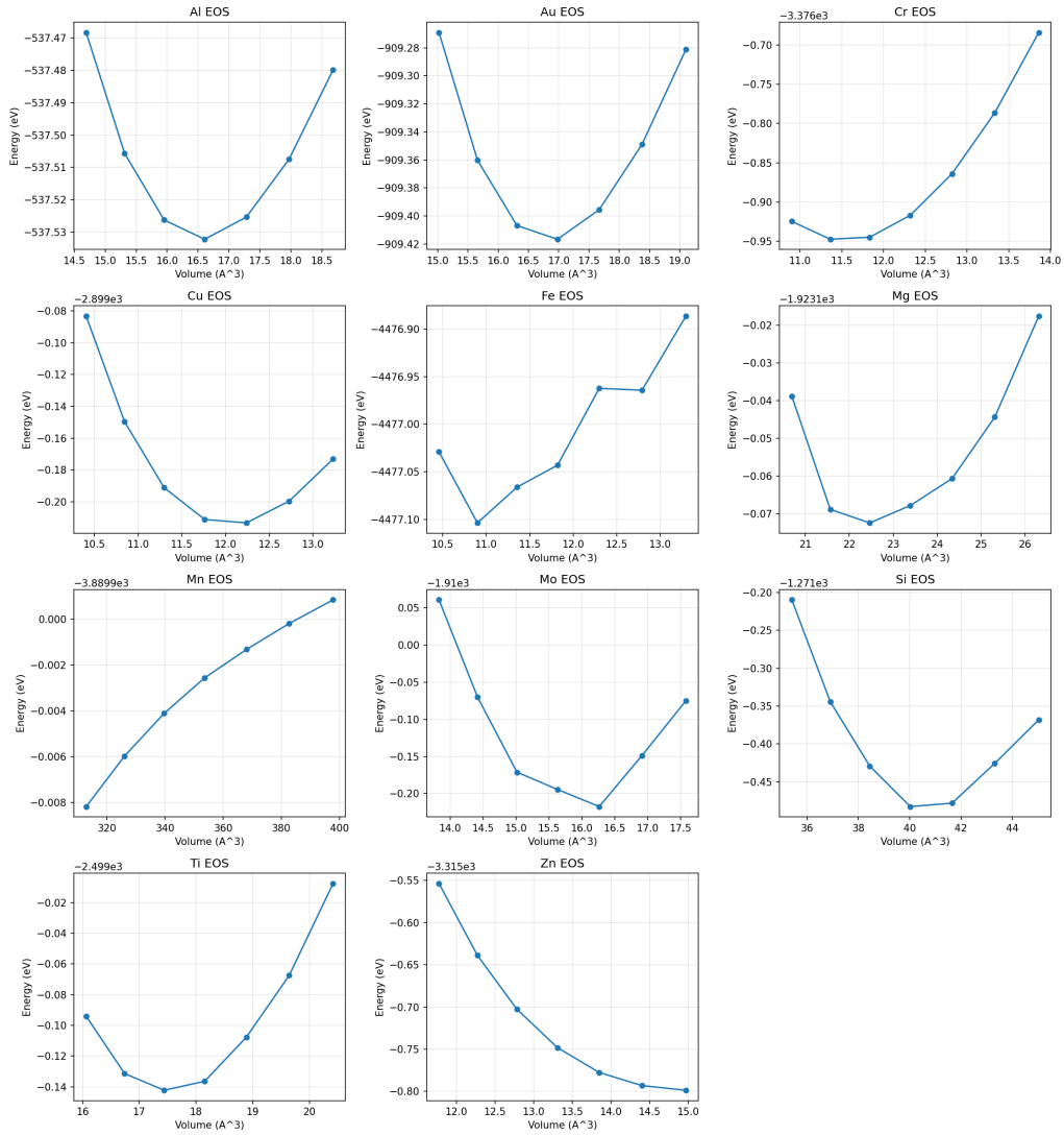
Figure 6: Birch–Murnaghan fits to the seven-point DFT equation-of-state scans. The fitted minimum sets a_0 and E_{\text{coh}} ; the curvature sets B .
