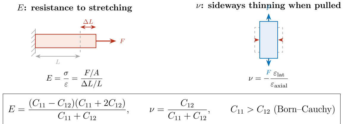
Figure 1: The two elastic moduli this work predicts. Left : a uniaxial force F stretches a bar by \Delta L , and the stiffness E = \sigma/\varepsilon is the stress-to-strain ratio. Right : the same axial pull makes the block contract laterally, and \nu is the negated ratio of lateral to axial strain. For a cubic crystal both reduce to the two independent stiffness constants C_{11} and C_{12} (boxed), and mechanical stability requires C_{11} > C_{12} .
