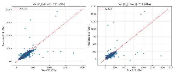
Figure 8: Held-out parity on the raw targets C_{11} and C_{12} , the quantities the network actually regresses.
