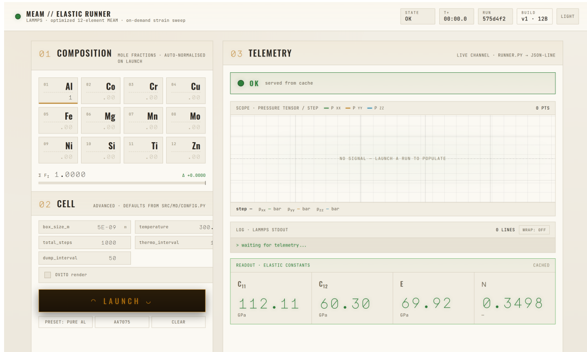
Figure 15: The MEAM elastic-runner app, shown on a pure-aluminium run against the optimized potential. The left column sets the composition and the supercell and run-length knobs; the right column streams the LAMMPS job and reports the elastic-constants readout. Here the run returns C_{11} = 112.1 GPa, C_{12} = 60.3 GPa, E = 69.9 GPa, and \nu = 0.350 .
