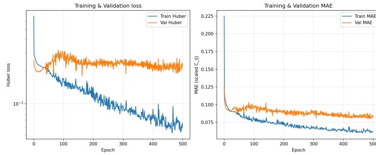
Figure 10: Training history of the composition surrogate: Huber loss and MAE on the scaled targets over training.
