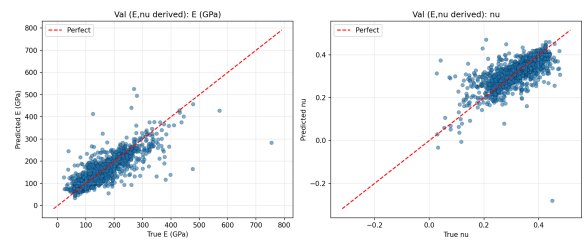
Figure 9: Held-out parity on the derived (E, \nu) , recovered from the predicted constants through Eq. (1).
