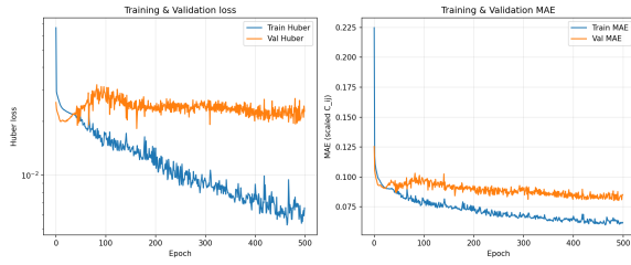
Figure 9: Training history: Huber loss and MAE on the scaled targets.
