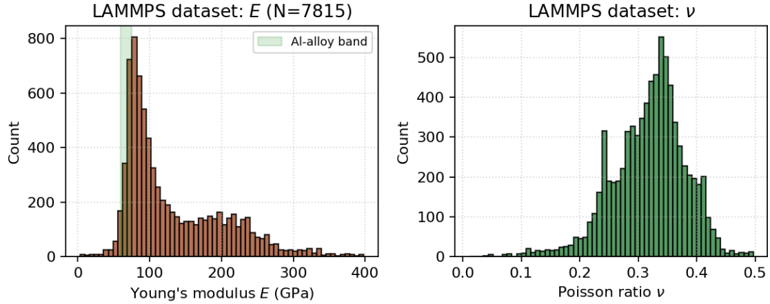
Figure 3: Histograms of E (left) and \nu (right) over the LAMMPS-evaluated dataset. The shaded band on the left panel marks the experimentally expected 60–75 GPa range for aluminium alloys, which contains 14.0 % of the physical sample.
