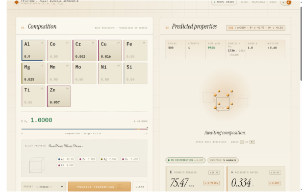
Figure 10: The surrogate packaged as a portable predictor. A composition is entered on the simplex and the ensemble returns (E, \nu) with a k -nearest-neighbour distance flag for out-of-distribution inputs.
