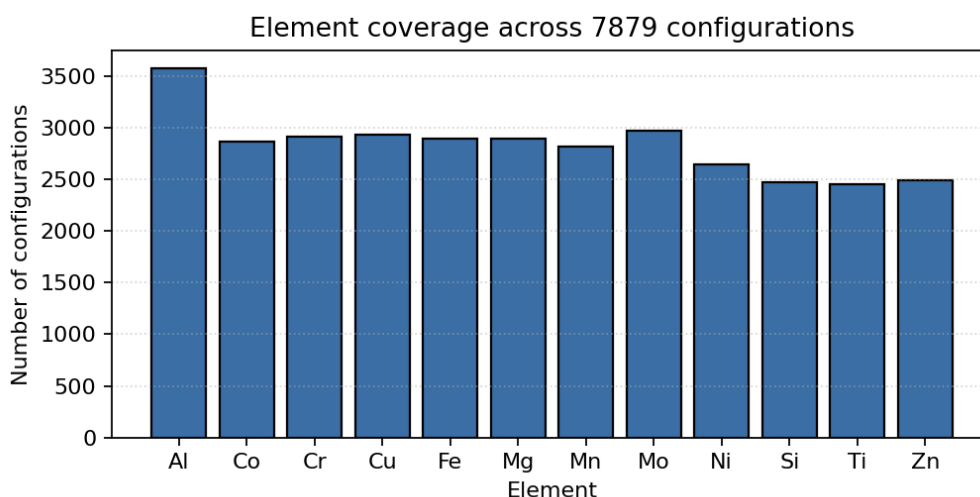
Figure 2: Number of configurations in which each element is present, over the retained corpus. The dominance of Al reflects the bias rule that keeps aluminium as the majority species whenever it is drawn.
