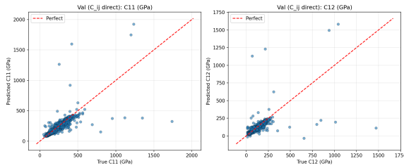
Figure 7: Held-out parity on the raw targets C_{11} and C_{12} , the quantities the network actually regresses.
