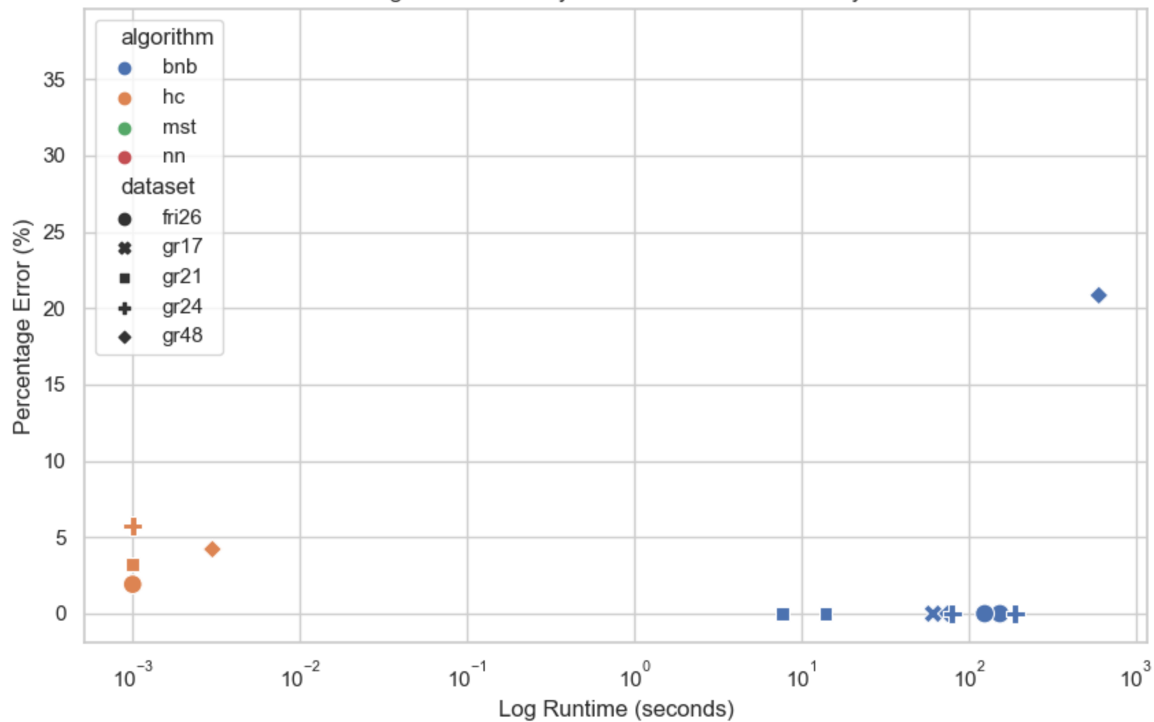
Algorithm Efficiency: Runtime vs Solution Quality
