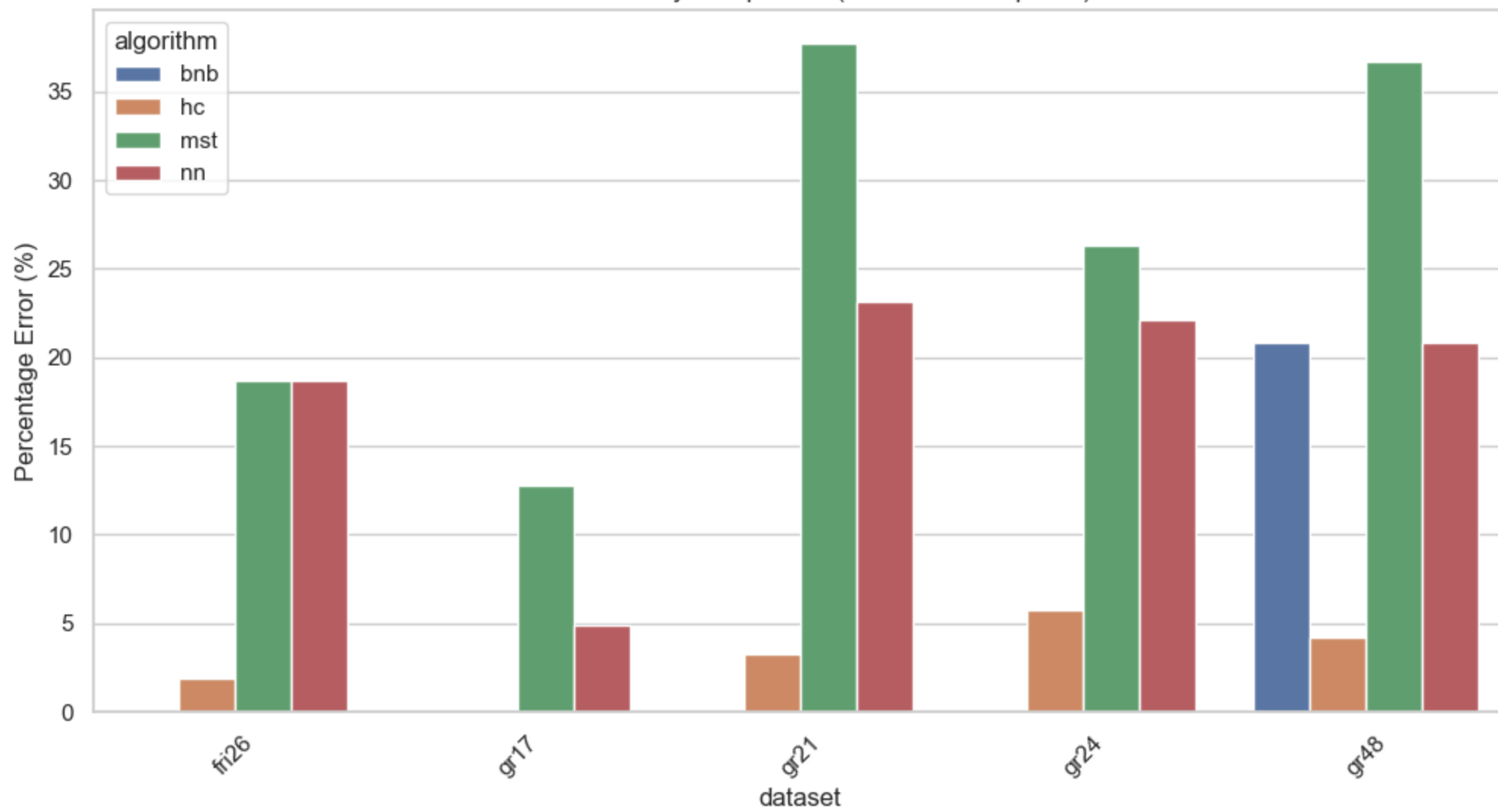
Solution Quality Comparison (% Error from Optimal)
