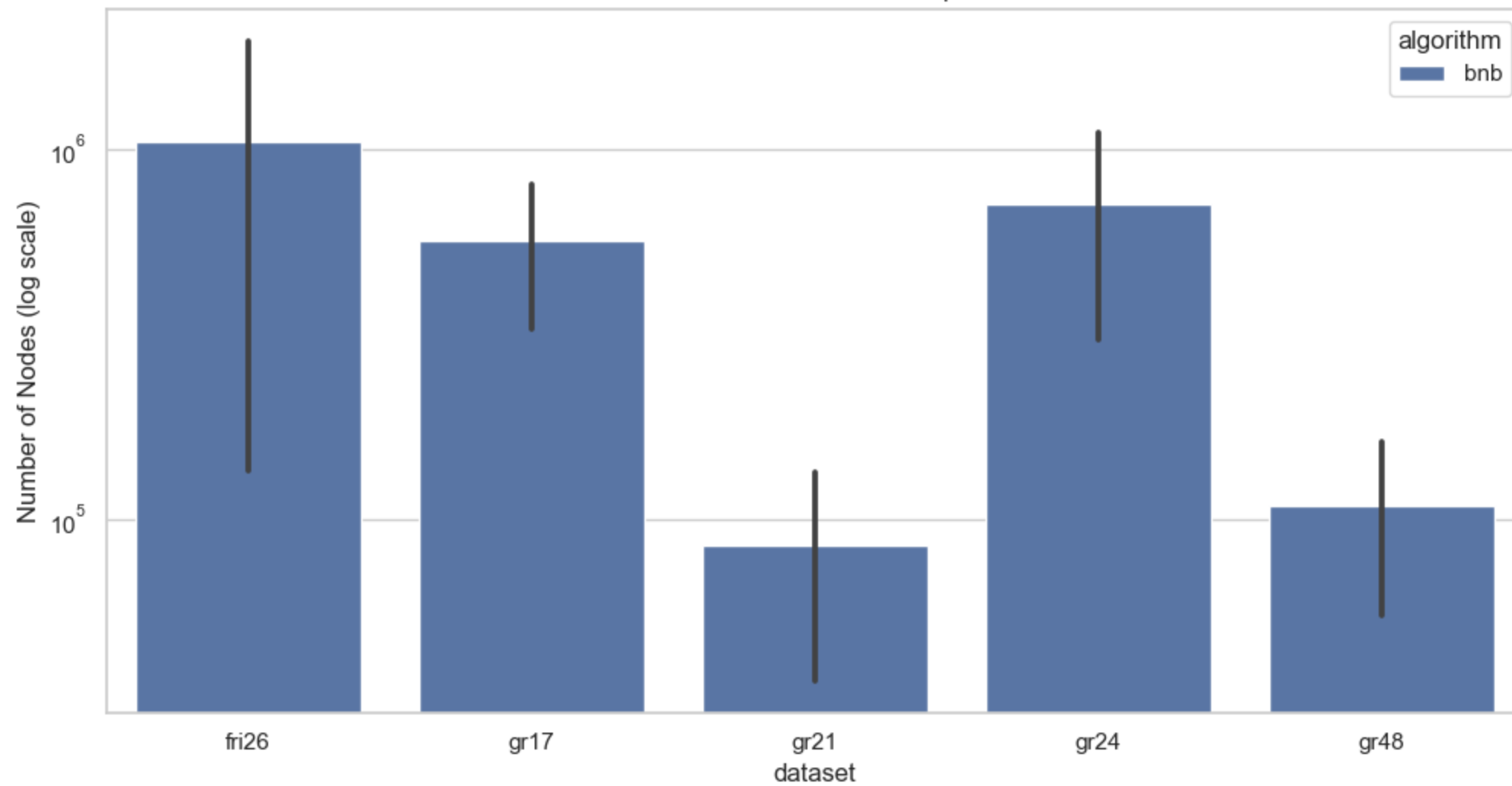
Branch and Bound Nodes Explored
