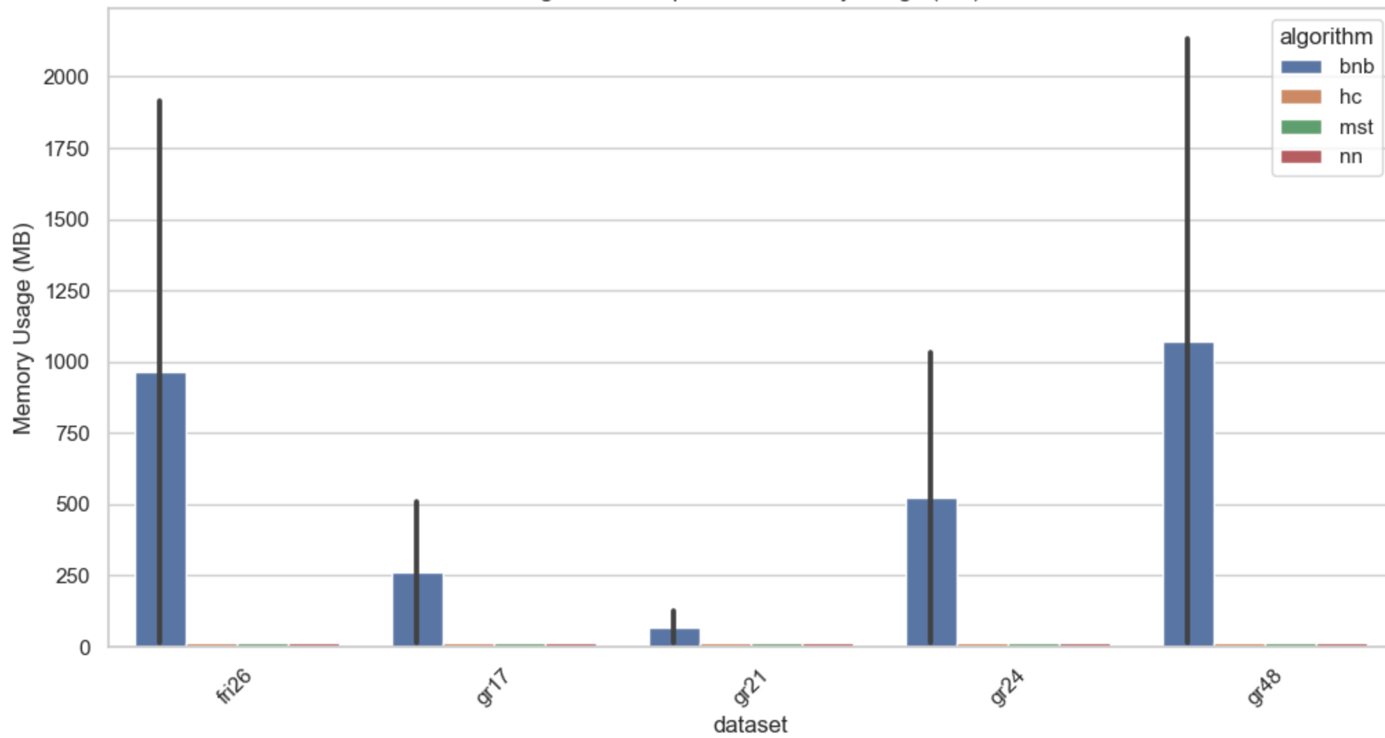
Algorithm Comparison - Memory Usage (MB)
