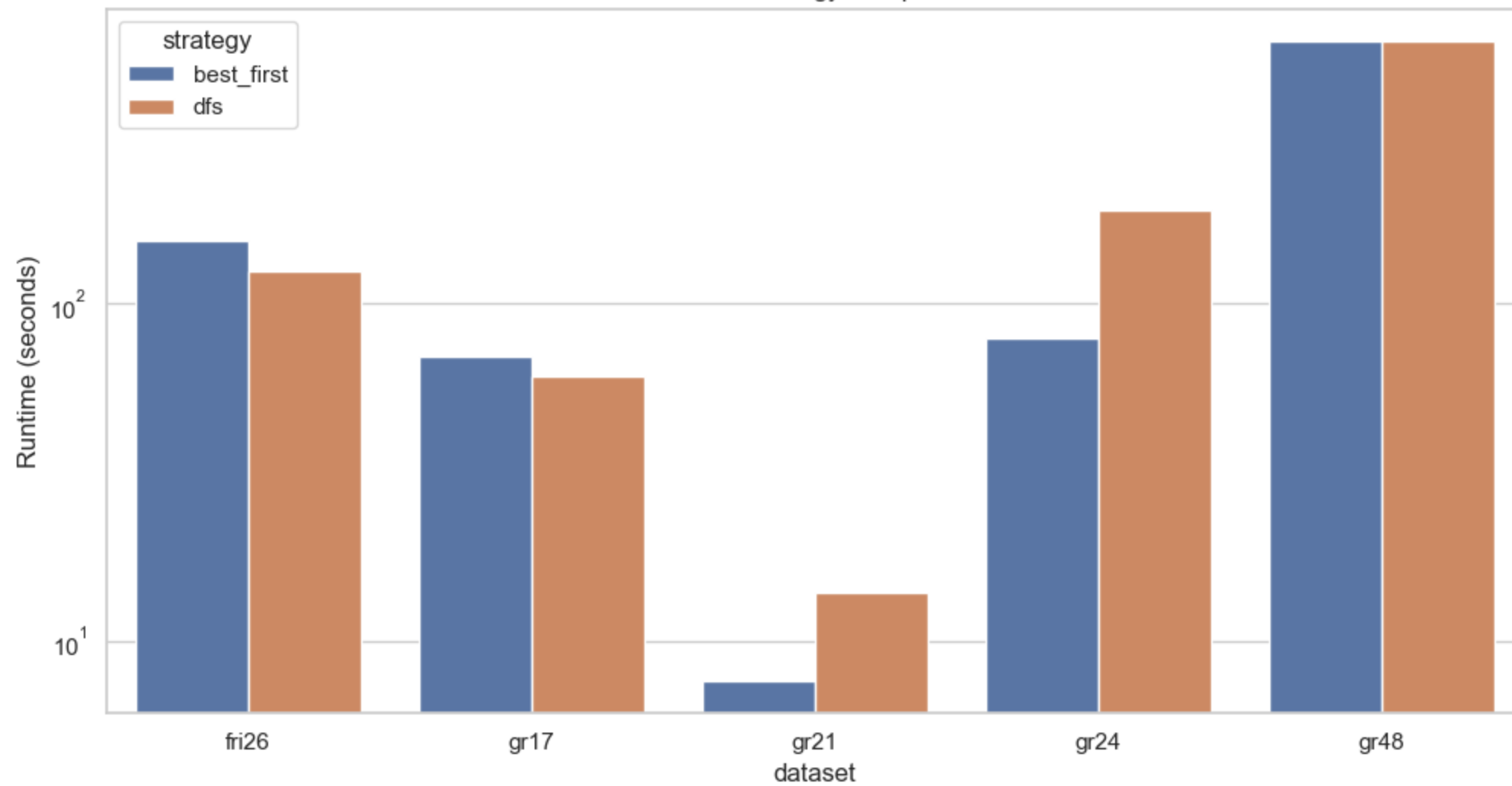
Branch and Bound Strategy Comparison - Runtime
