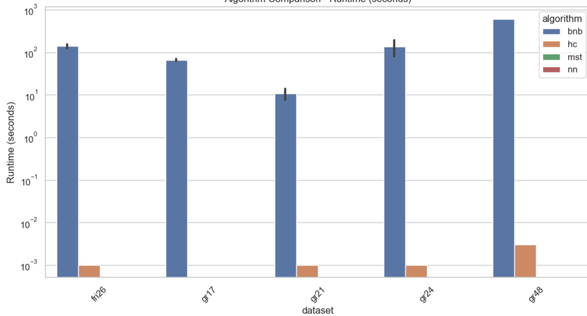
Algorithm Comparison - Runtime (seconds)
