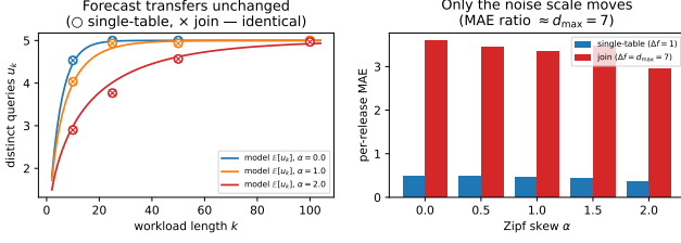
Figure 7: Twin single-table vs. join experiment (TPC-H, m=5 priority pool, d_{\max}=7 , 600 trials). Left: the realized distinct count for the single-table (○) and join (×) workloads lands on the same analytical \mathbb{E}[u_k] curve. Right: only the per-release noise scale moves, by \Delta f (1 vs d_{\max}=7 ).
