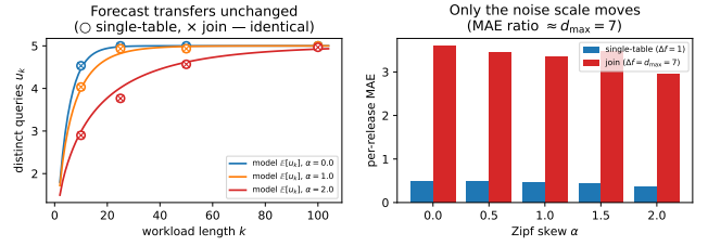
Figure 6: Twin single-table vs. join experiment (TPC-H, m=5 priority pool, d_{\max}=7 , 600 trials). Left: the realized distinct count for the single-table (○) and join (×) workloads lands on the same analytical \mathbb{E}[u_k] curve—the forecast transfers unchanged. Right: only the per-release noise scale moves, by \Delta f (1 vs d_{\max}=7 ).
