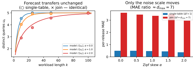
Figure 7: Twin single-table vs. join experiment (TPC-H, m=5 priority pool, d_{\max}=7 , 600 trials). Left: the realized distinct count for the single-table (○) and join (×) workloads lands on the same analytical \mathbb{E}[u_k] curve. Right: only the per-release noise scale moves, by \Delta f (1 vs d_{\max}=7 ).
