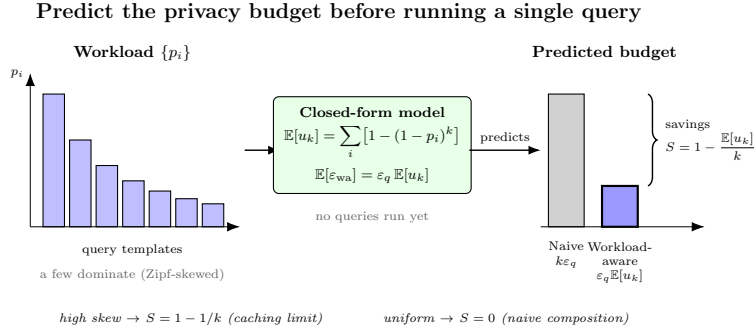
Fig. 1. Naive composition charges every one of k queries; workload-aware accounting charges only the u_k distinct query species, since exact repeats are served from cache by post-processing. The model predicts \mathbb{E}[u_k] , and hence the budget, before execution.
