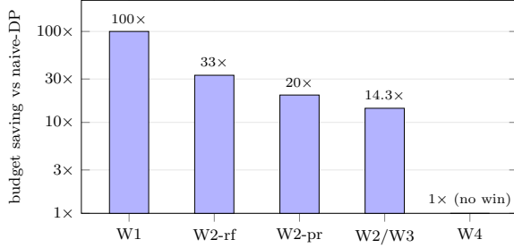
Figure 5: Budget saved versus the naive-DP baseline, per workload ( k = 100 , \varepsilon_q = 1 , log scale). Workload-aware accounting answers the same queries while spending only \varepsilon_q \cdot u_k : up to 100\times less on the repetitive W1 and 14\text{--}33\times less on the parametric/uniform pools, but exactly 1\times (no win) on the genuine drill-down W4, where every query is unique and the model predicts S(k) = 0 .
