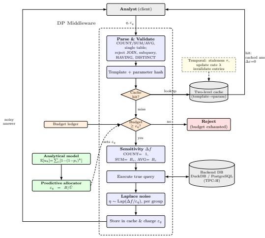
Figure 2: Architecture of the workload-aware DP-SQL middleware. Each query is parsed, hashed, and checked against a two-level cache; a cache hit is returned for free by post-processing, while a miss is charged \epsilon_q against the budget ledger, noised by the Laplace mechanism, and cached. The analytical model drives the predictive allocator that sets \epsilon_q = B/\hat{U} online, and a temporal regime (\tau, \lambda) invalidates stale cache entries.
