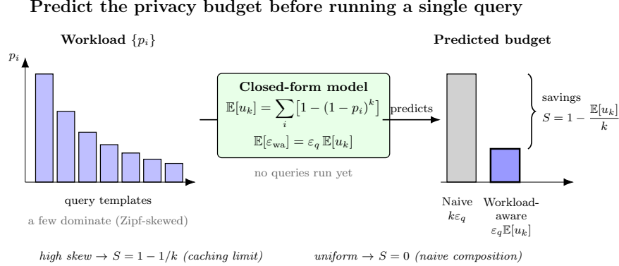
Fig. 1. Naive composition charges every one of k queries; workload-aware accounting charges only the u_k distinct query species, since exact repeats are served from cache by post-processing. The model predicts \mathbb{E}[u_k] , and hence the budget, before execution.
