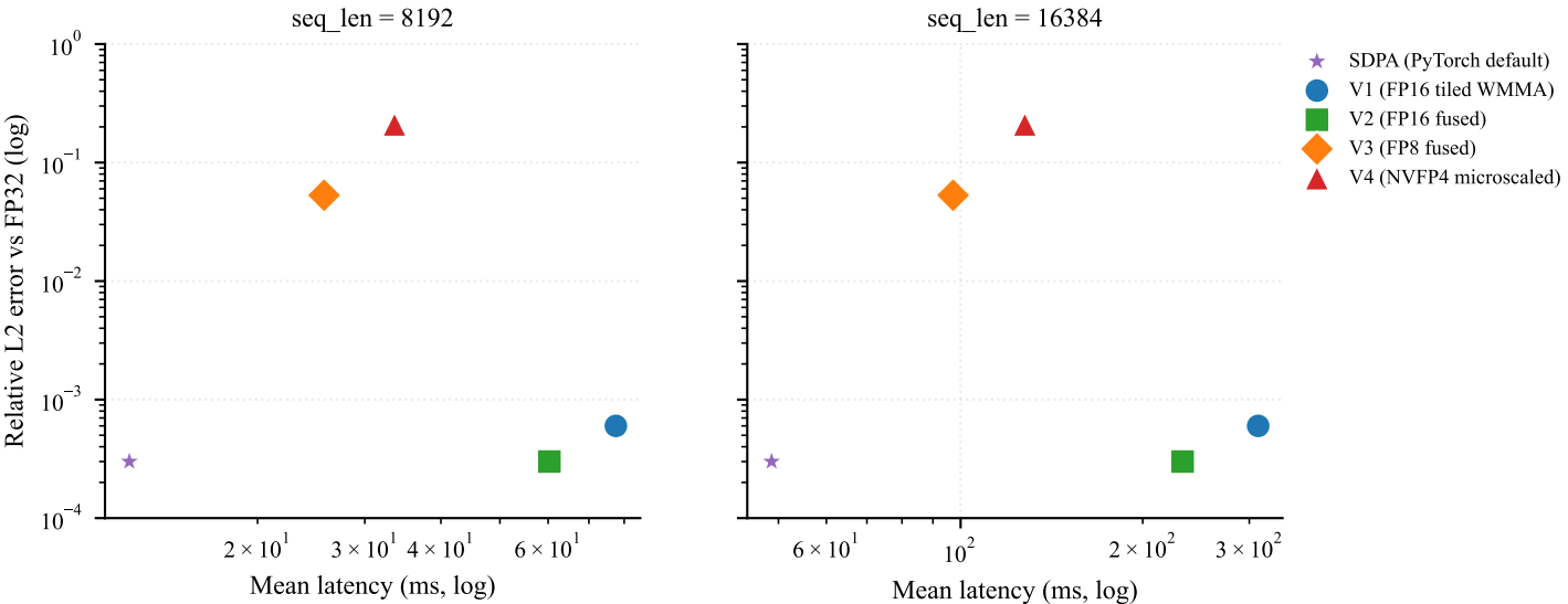
Latency--accuracy Pareto on RTX 5080 (head_dim=128, batch=2, heads=8)
