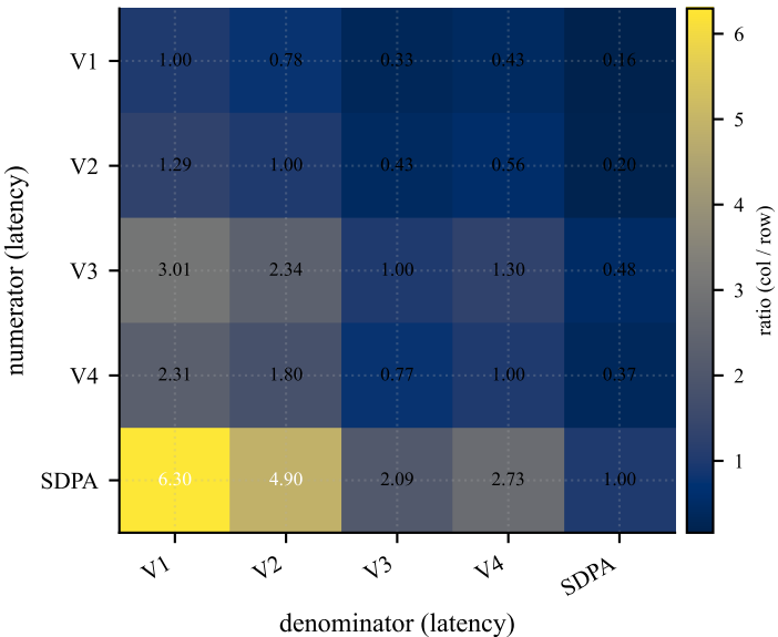
Pairwise speedup at seq_len=8192, head_dim=128
