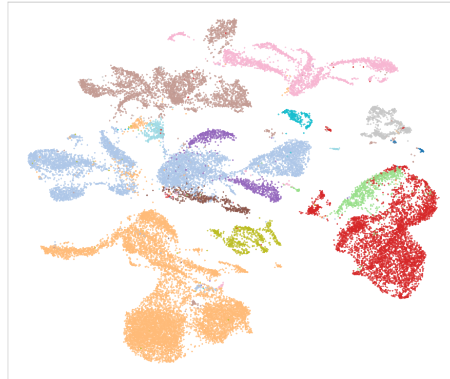
TranscriptFormer Metazoa
