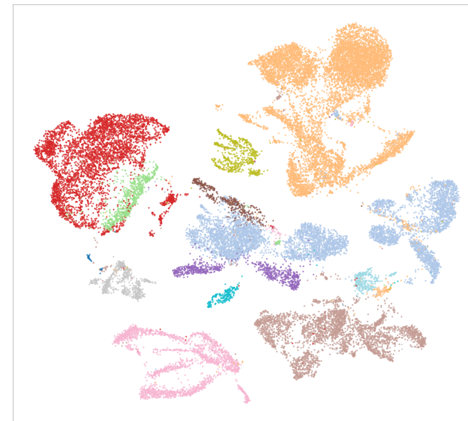
TranscriptFormer Metazoa
