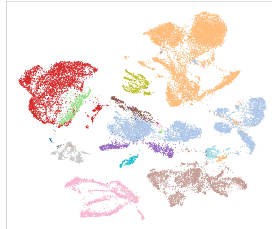
TranscriptFormer Metazoa
