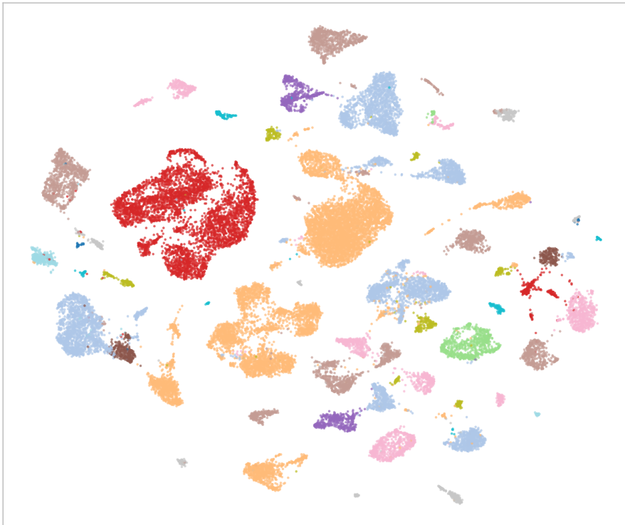
Expression PCA50
