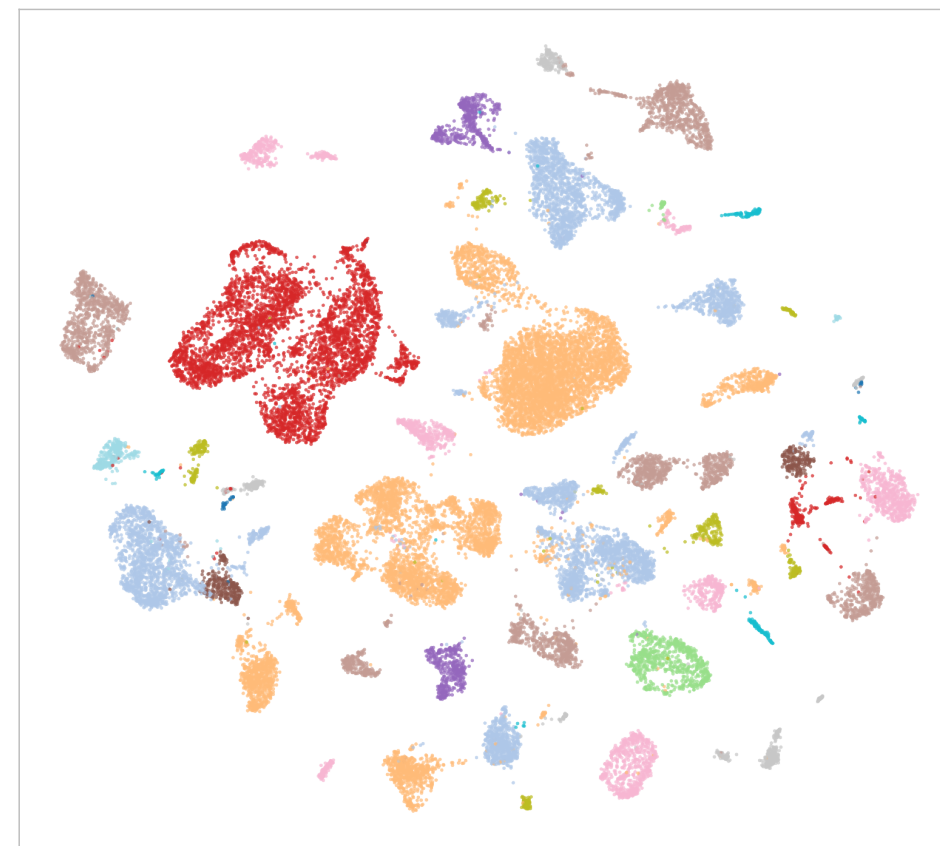
Expression PCA50
