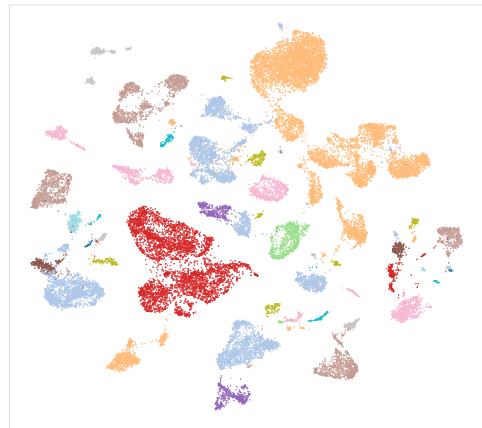
Expression PCA50
