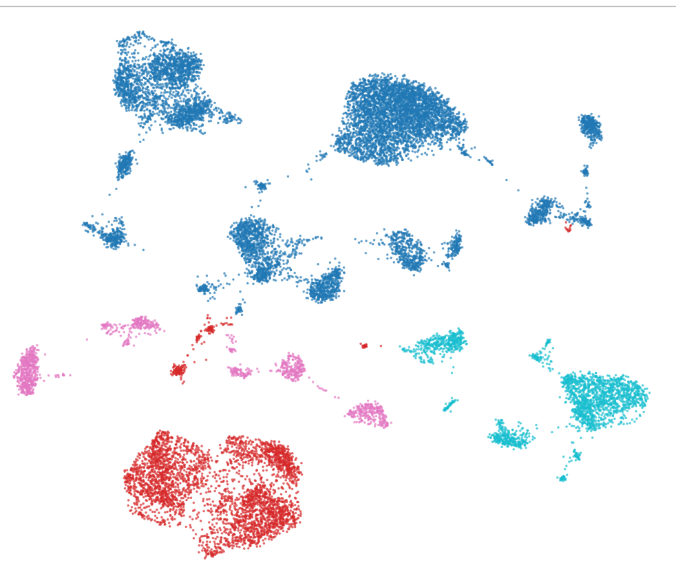
Expression PCA50
