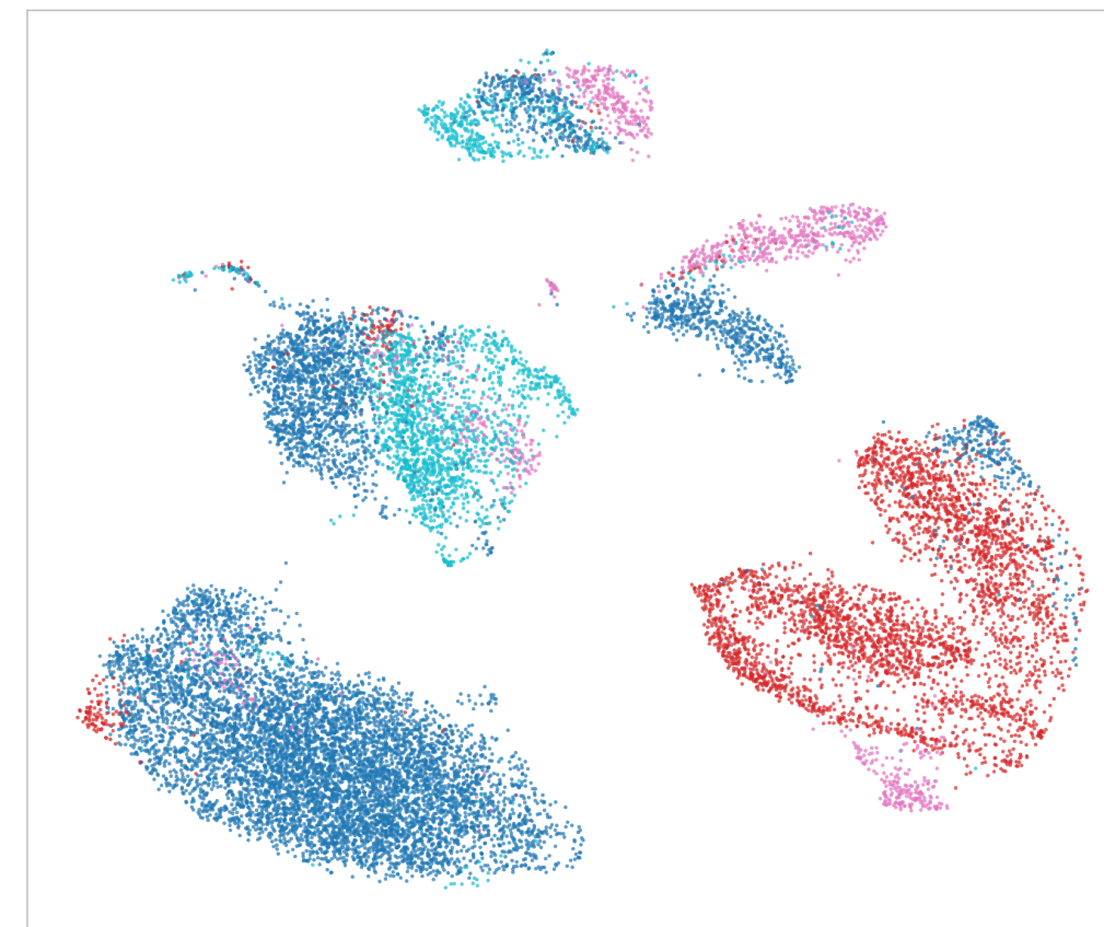
TranscriptFormer Metazoa
