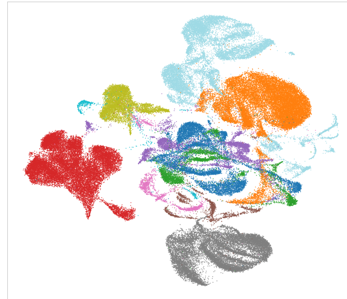
TranscriptFormer Metazoa
