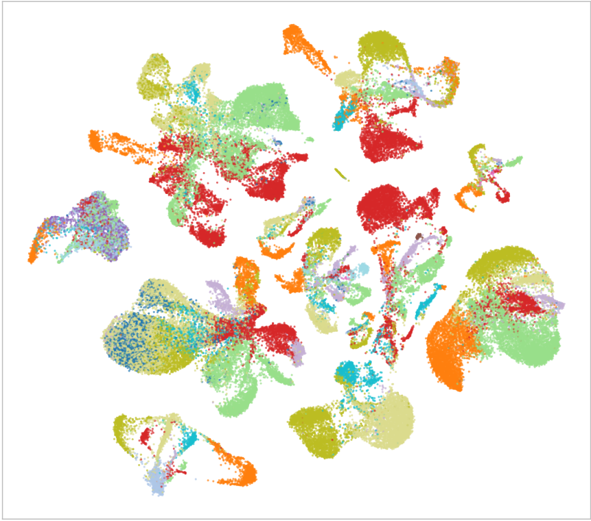
Expression PCA50
