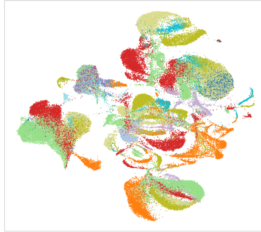
TranscriptFormer Metazoa
