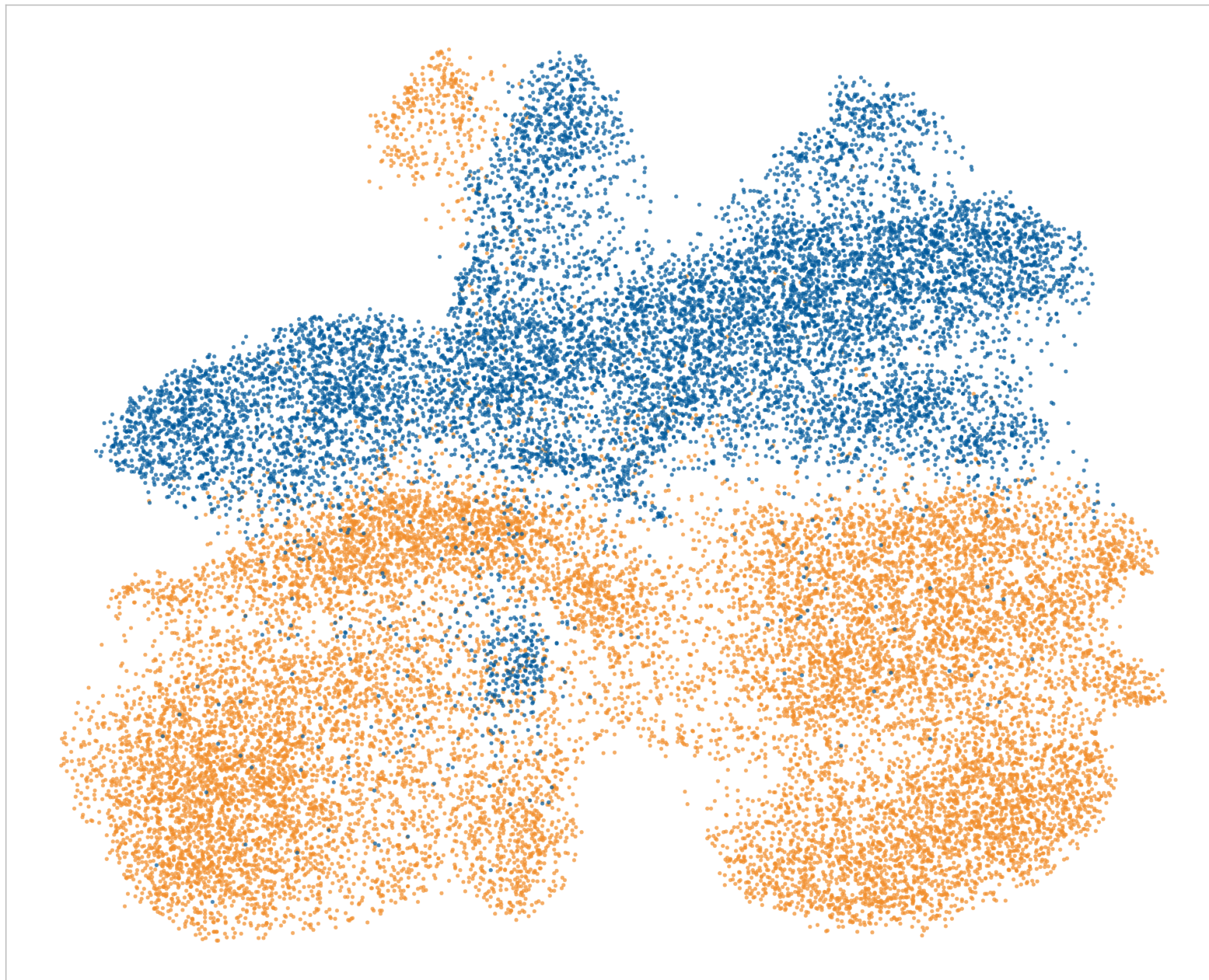
scPRINT-2 — Species
