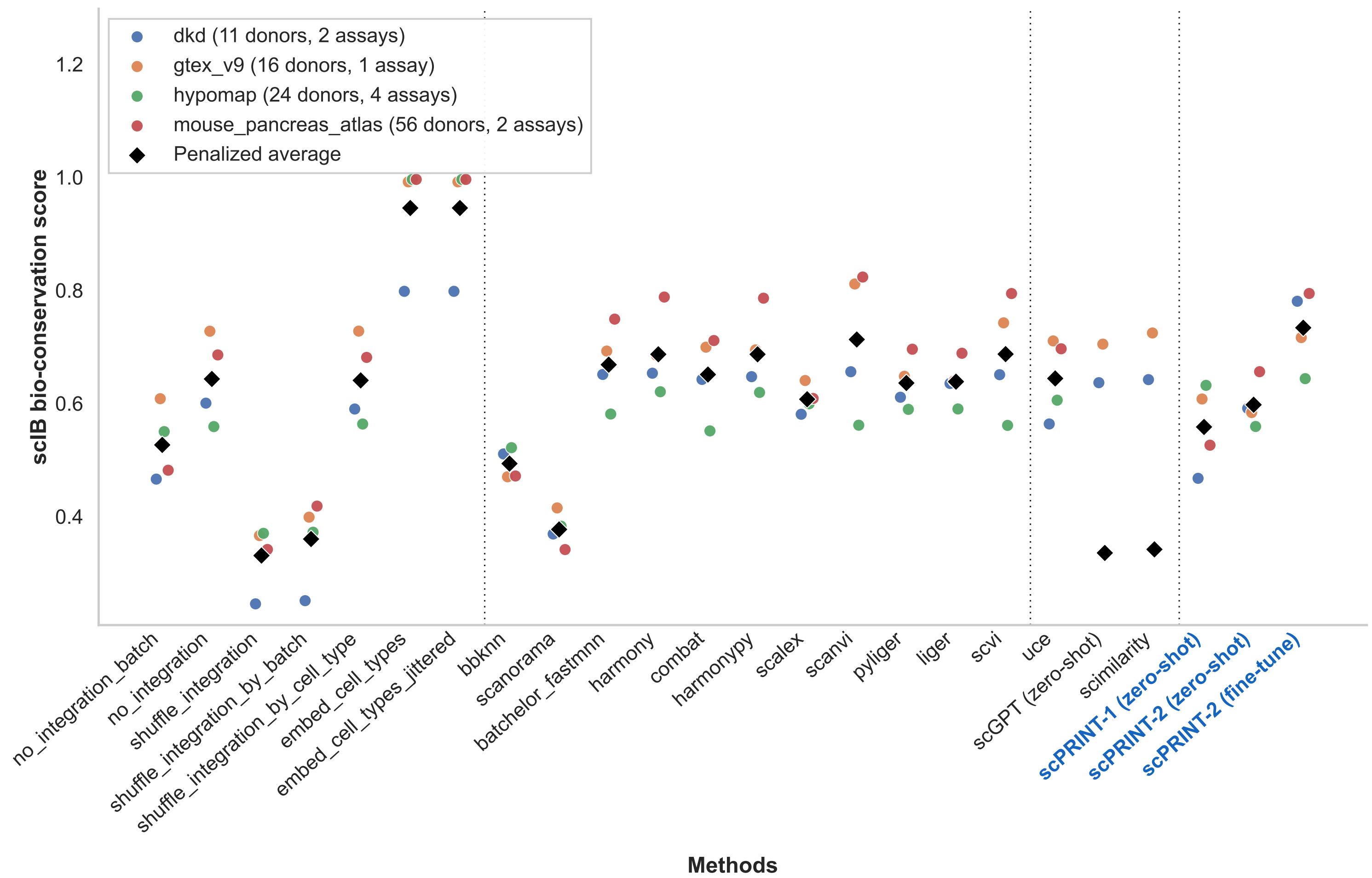
OpenProblems batch integration: Bio conservation black diamond = penalized average; dots = raw score per dataset; missing scores set to 0
