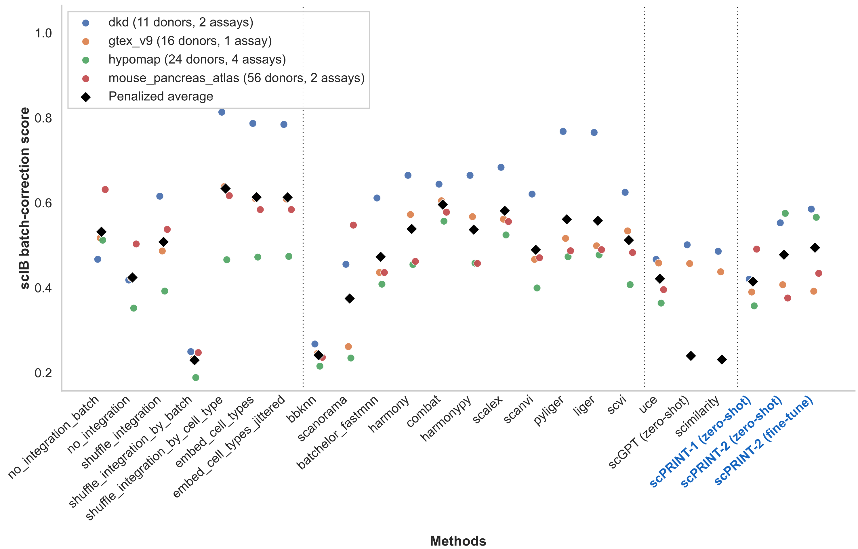
OpenProblems batchintegration: Batch correction black diamond = penalized average; dots = raw score per dataset; missing scores set to 0
