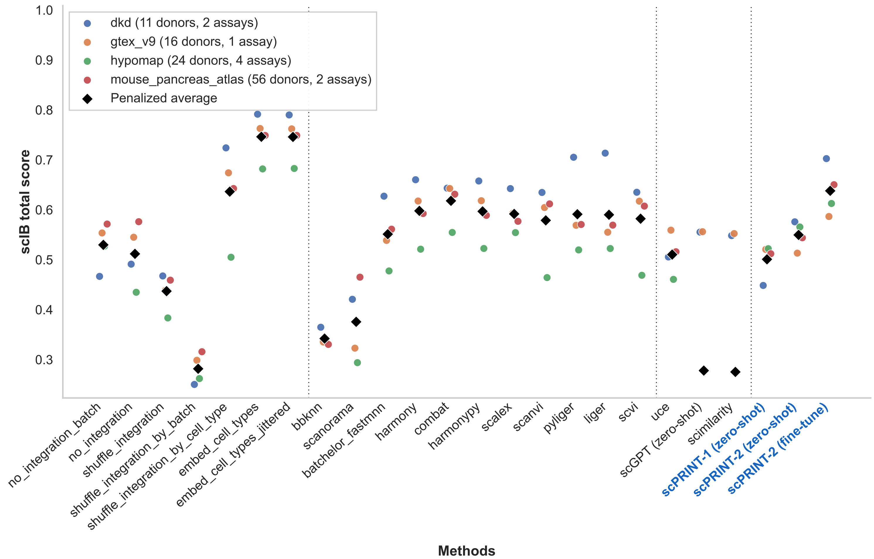
OpenProblems batch integration: Total black diamond = penalized average; dots = raw score per dataset; missing scores set to 0
