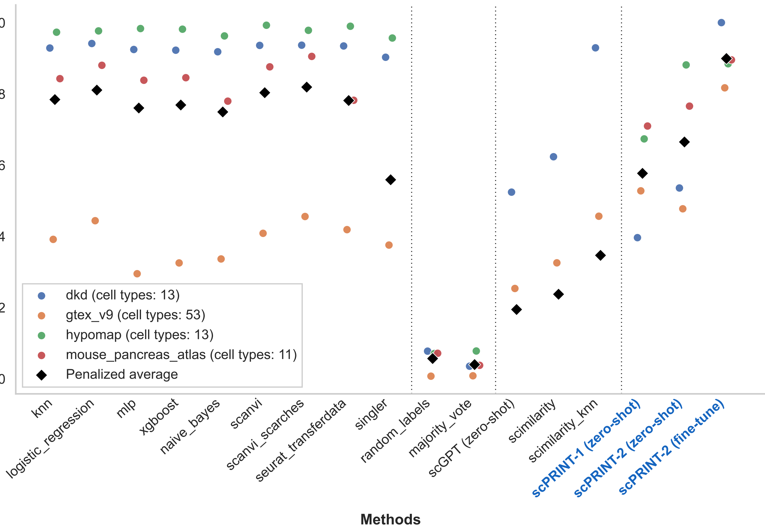
OpenProblems label projection: Macro F1 black diamond = penalized average; dots = raw score per dataset; missing scores set to 0
