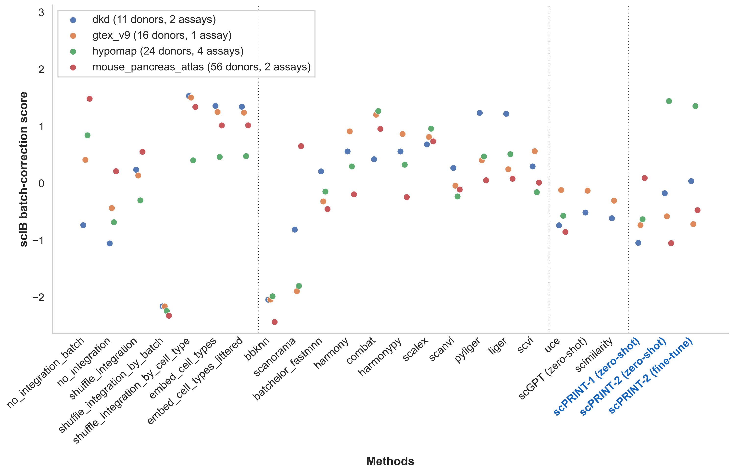
OpenProblems batch integration: Batch correction dots = z-score per dataset; missing scores excluded
