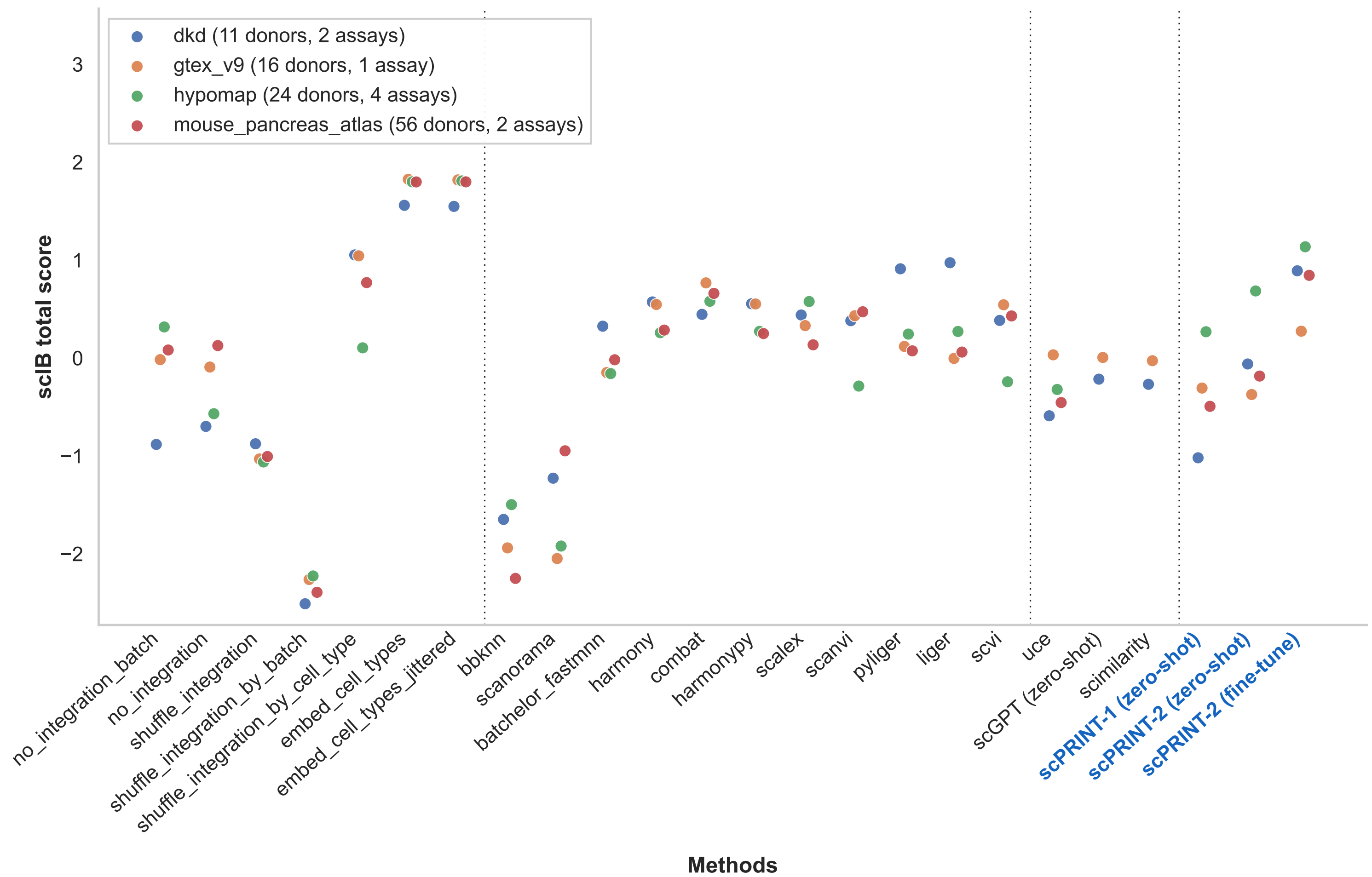
OpenProblems batch integration: Total dots = z-score per dataset; missing scores excluded
