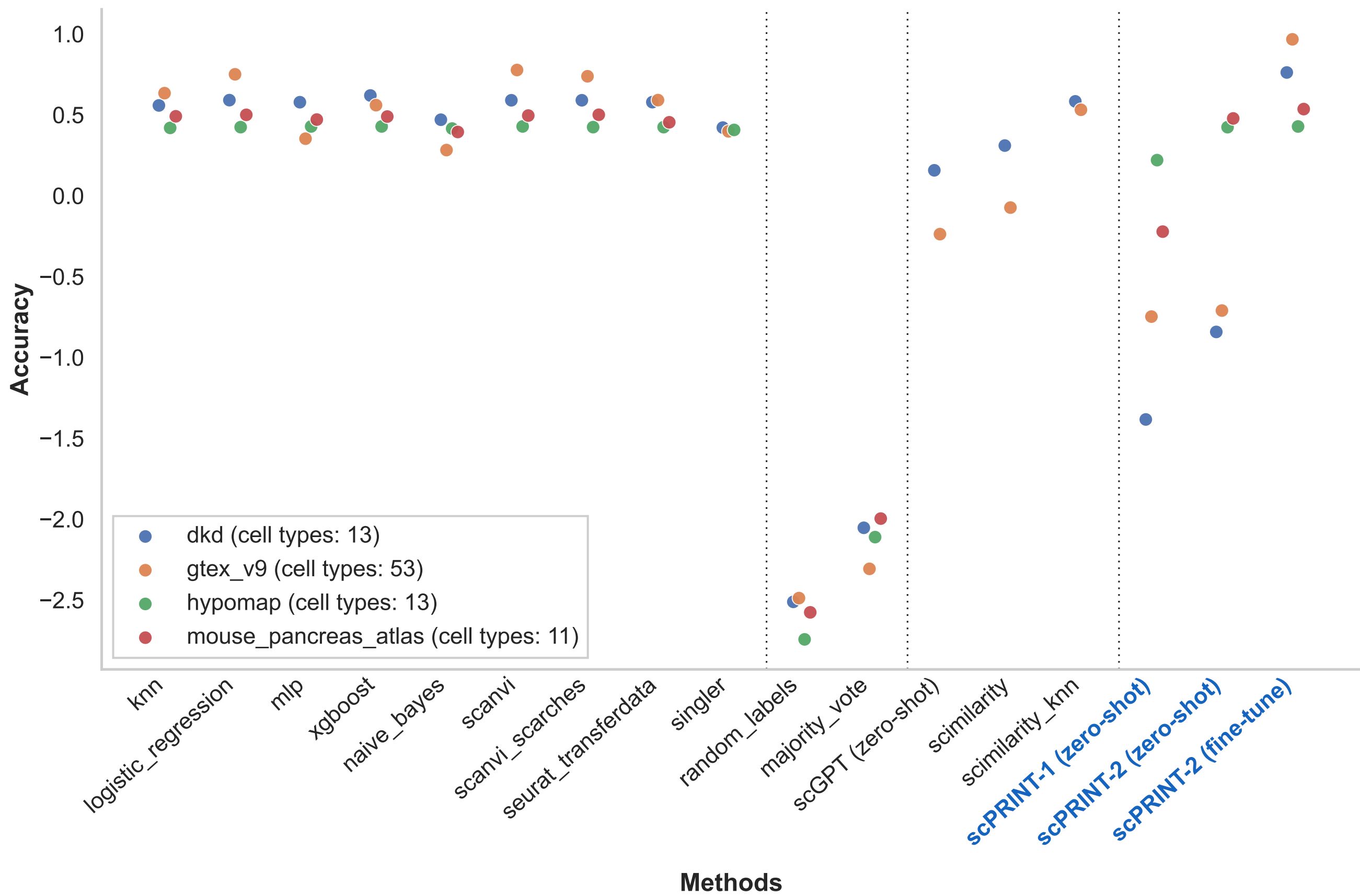
OpenProblems label projection: Accuracy dots = z-score per dataset; missing scores excluded
