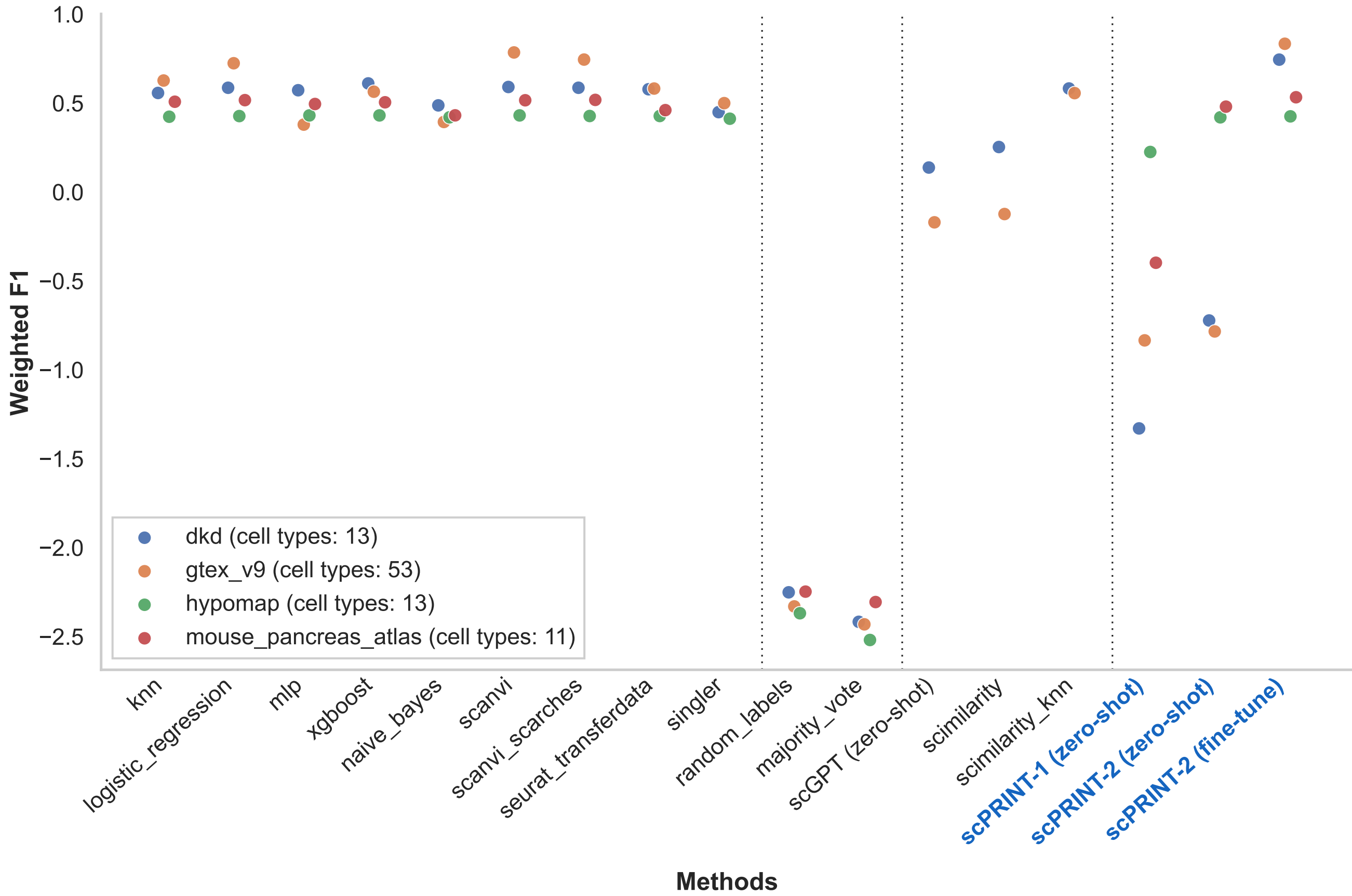
OpenProblems label projection: Weighted F1 dots = z-score per dataset; missing scores excluded
