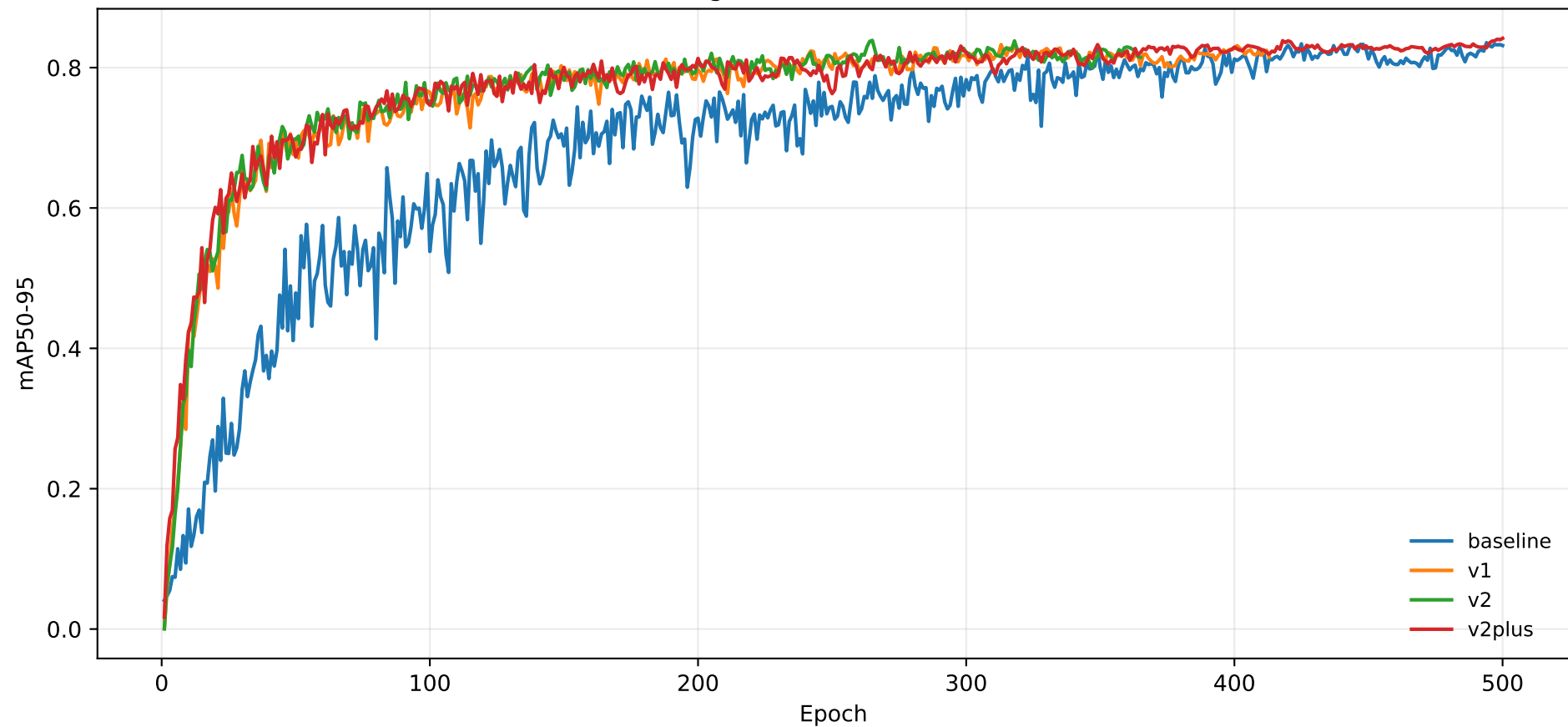
Convergence curve of mAP50-95
