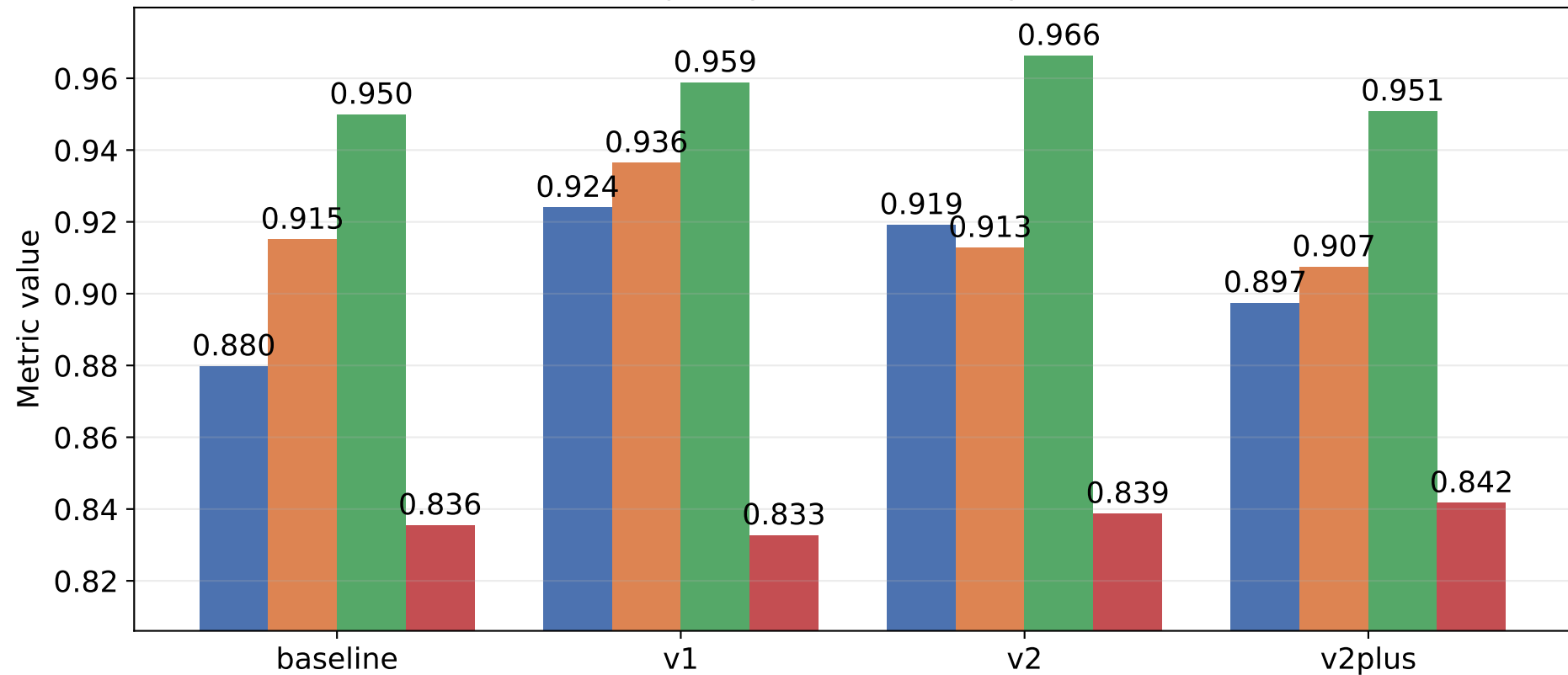
Precision Recall mAP50 mAP50-95 Best-point performance comparison
