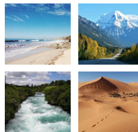
Natural scenes
