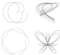
Geometric figures
