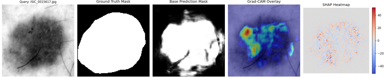
Figure 1: ISIC case ISIC_0015617. Grad-CAM (macro) : a single contiguous warm blob covers the body of the pigmented lesion, confirming the model attends to the lesion interior rather than the surrounding skin or the thin hair artifacts. GradientSHAP (micro) : a dense cloud of signed points tiles the same lesion territory; positive (red) responses concentrate on the darker, high-pigment texture that drives foreground probability up, while scattered blue points mark locally suppressive pixels. The two maps co-localize with the prediction, qualitative evidence of faithful attention.
