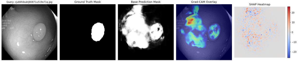
Figure 4: Kvasir case cju84hibuktj80871u519e71q.jpg , a diagnostic example. The ground-truth polyp (column 2) is small, yet the base prediction over-segments a large portion of the frame. Grad-CAM reveals why : its hot-spot sits above/left of the true polyp, on bright mucosal folds that the model has confused for lesion tissue. GradientSHAP spreads signed energy broadly rather than tightly, with mixed red/blue noise over the over-segmented area. Here the two explanations agree that the model is responding to spurious high-contrast mucosa—an interpretable account of a segmentation failure.
