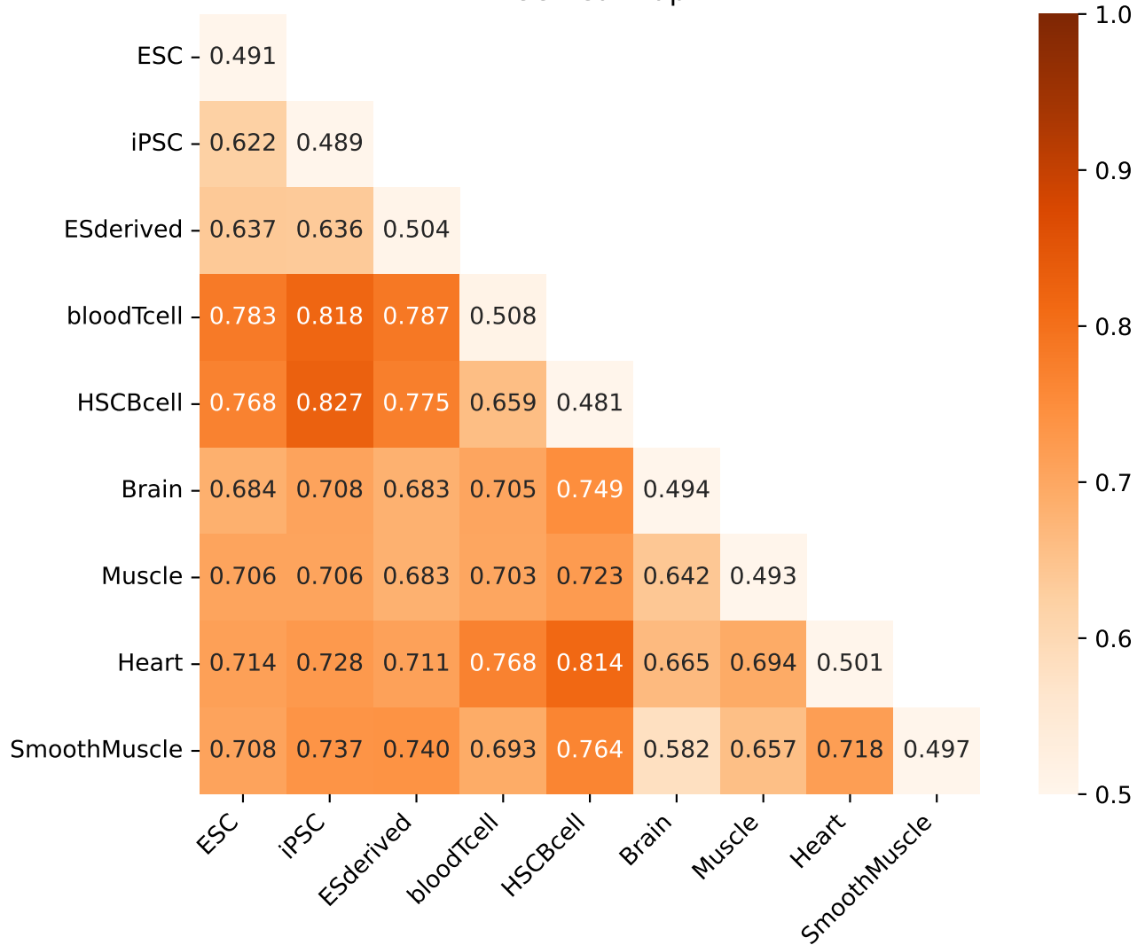
ACC heatmap
