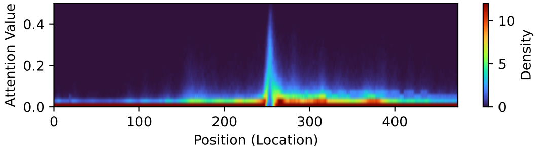
Attention Value Distribution Across Locations
