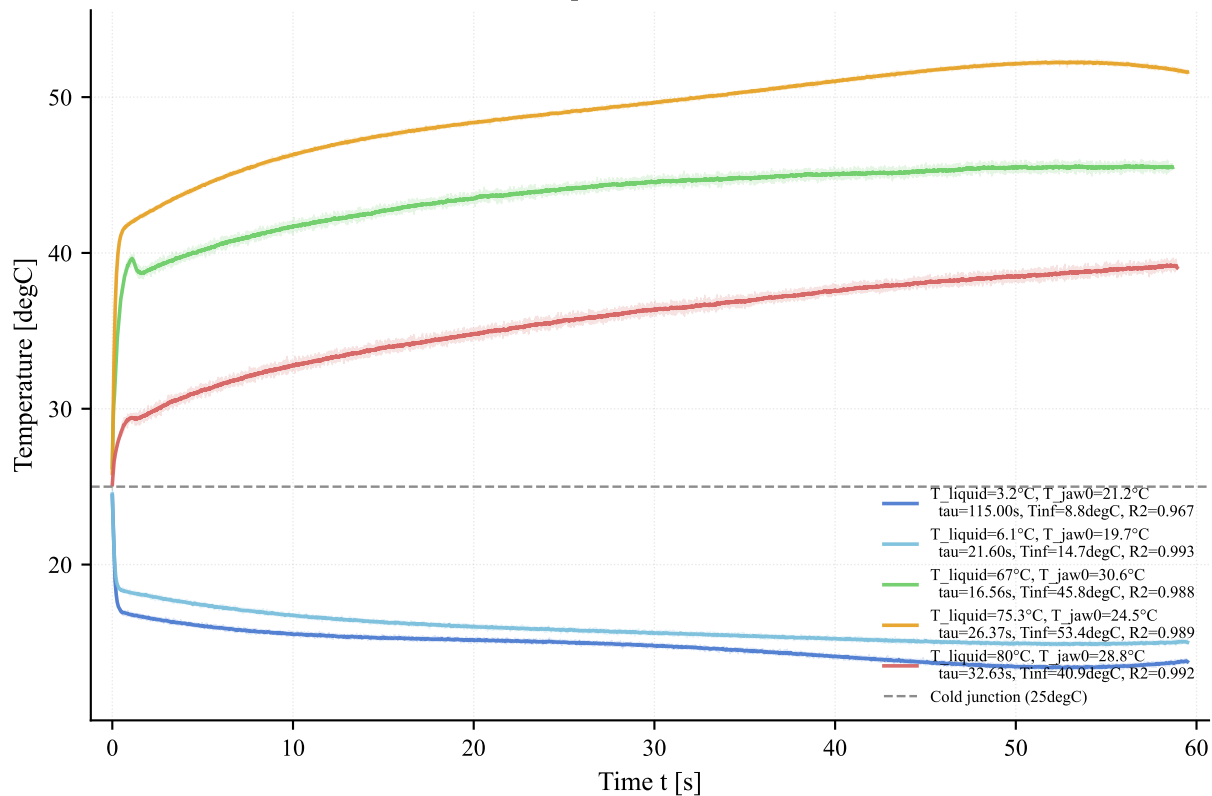
P0 temperature time curves
