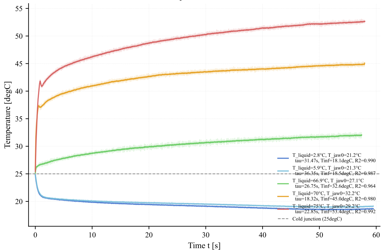
P1 temperature time curves
