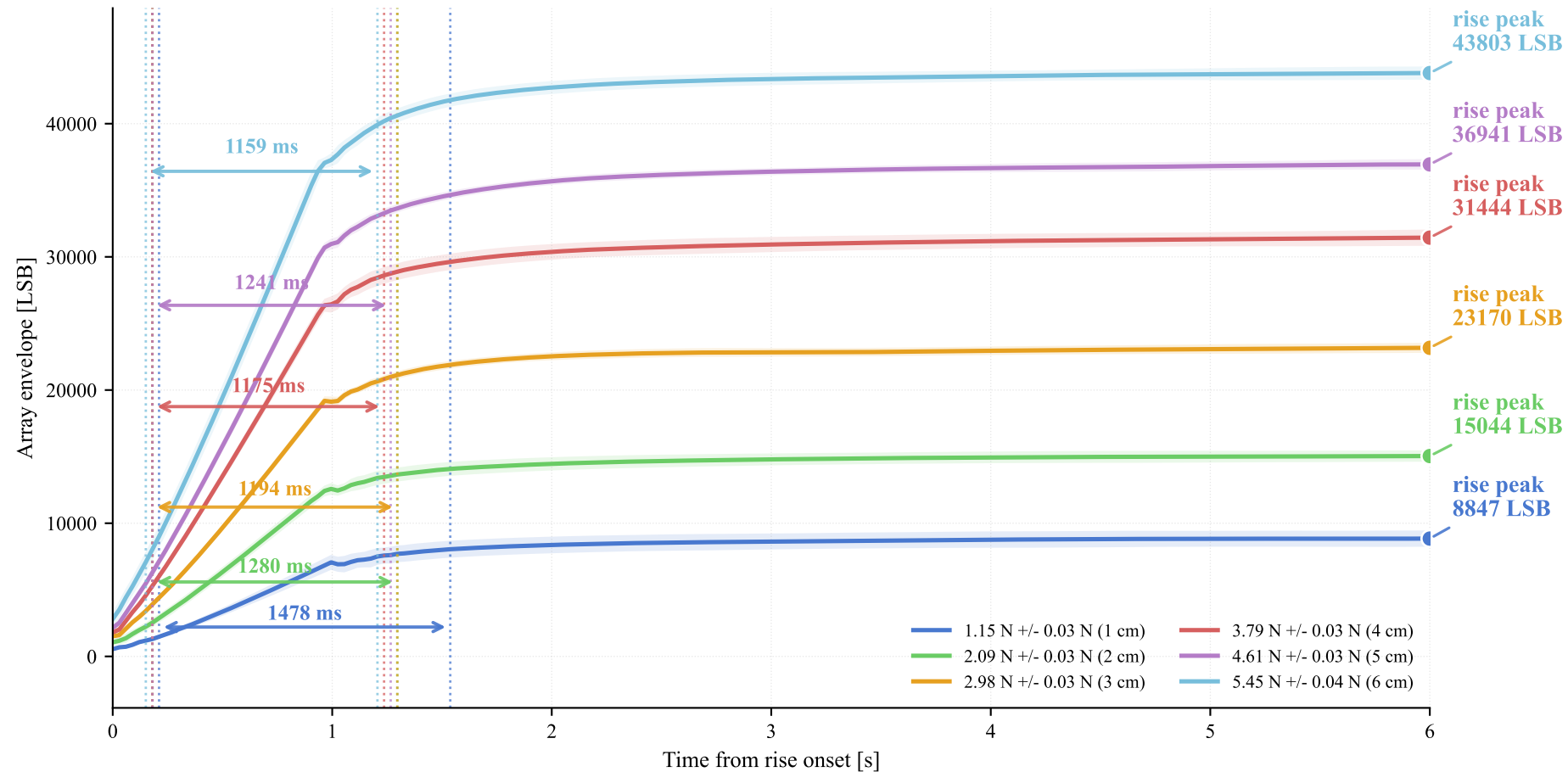
09a tactile force rising curves with rise time and peak point
