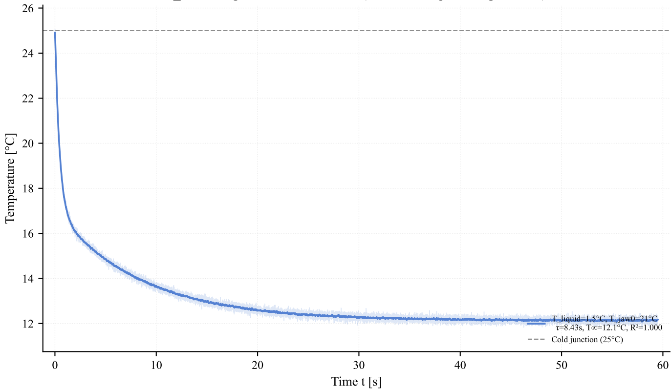
1_cold Temperature Time Curves (Different Liquid Temperatures)
