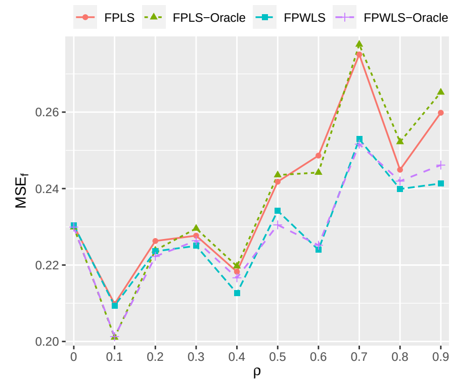
AR error with sample size n=400
