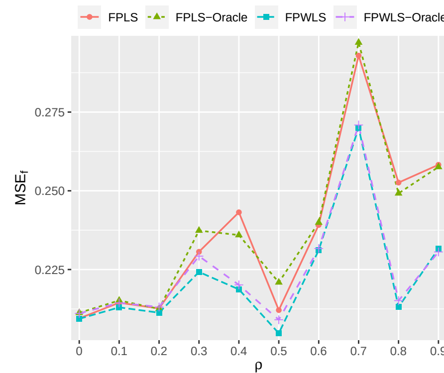
EX error with sample size n=400
