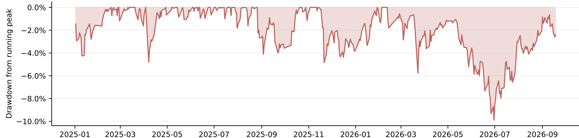
V3 rolling LightGBM + risk budget | 417 sessions, first-day loss included
