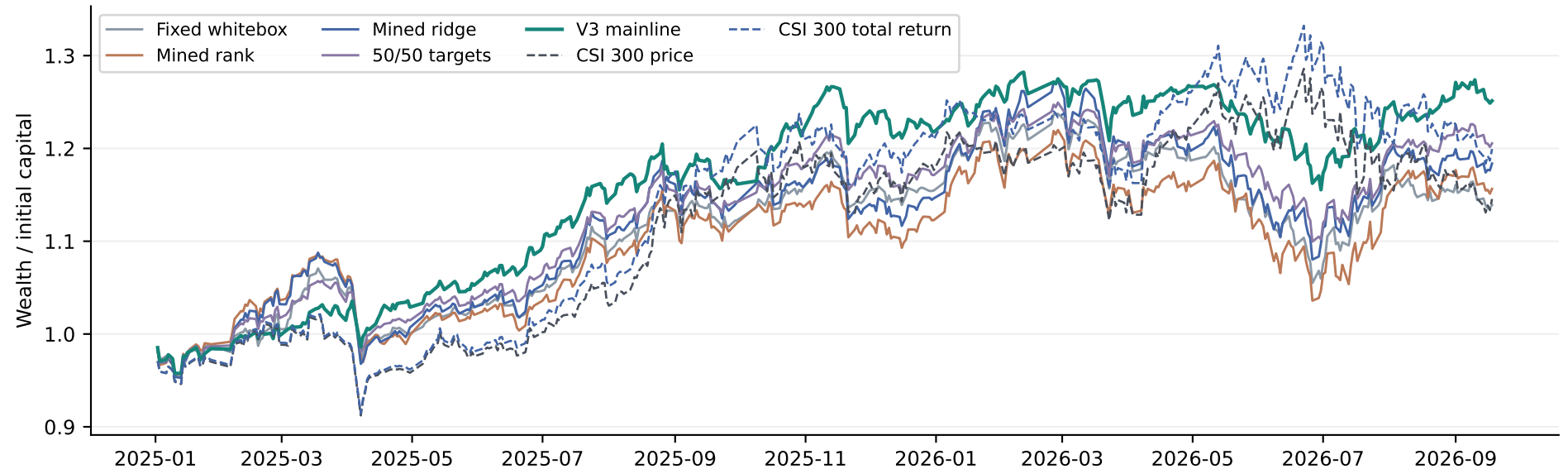
Same observed sessions and initial capital; actual costs included
