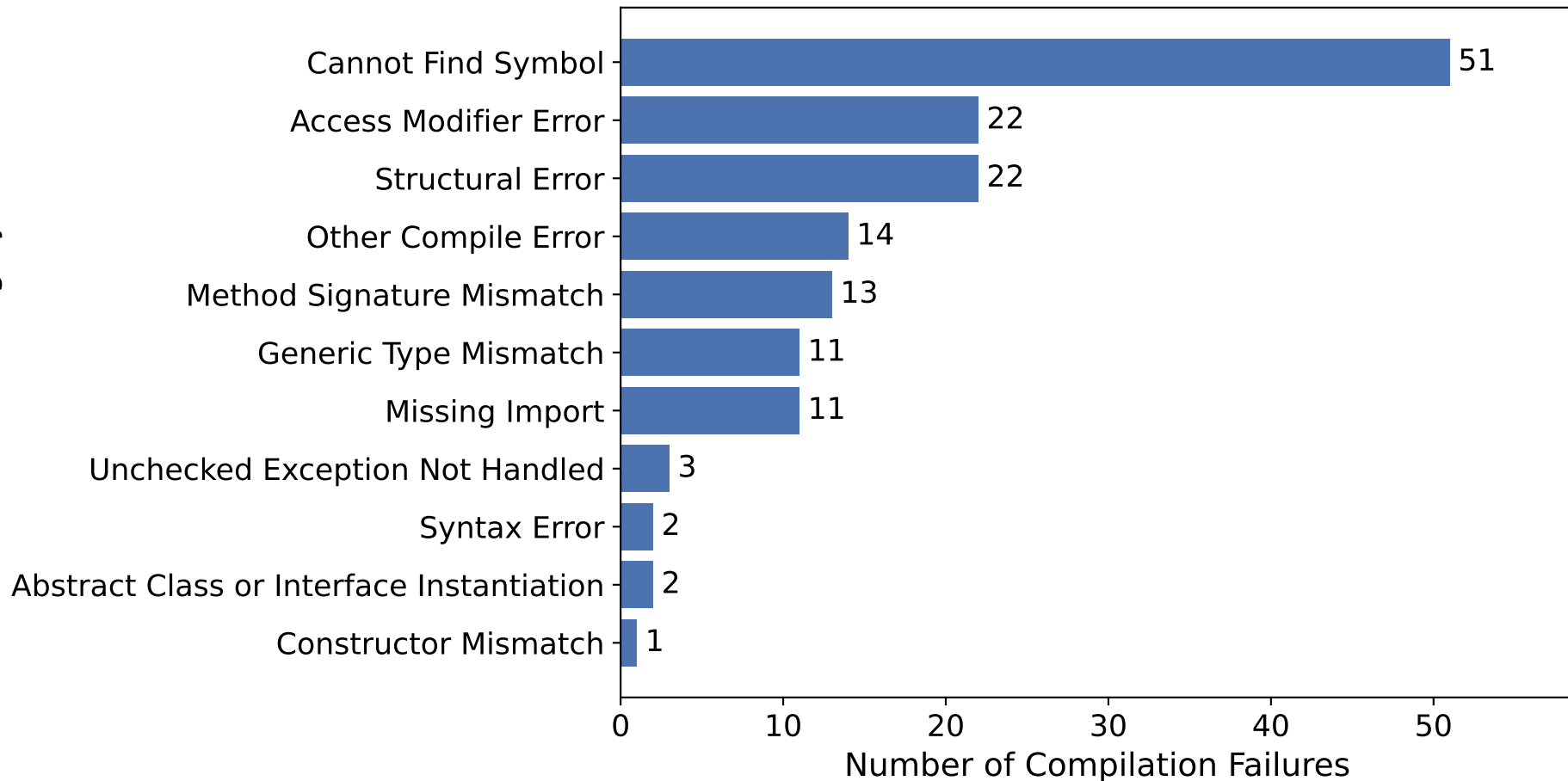
Failure Category
