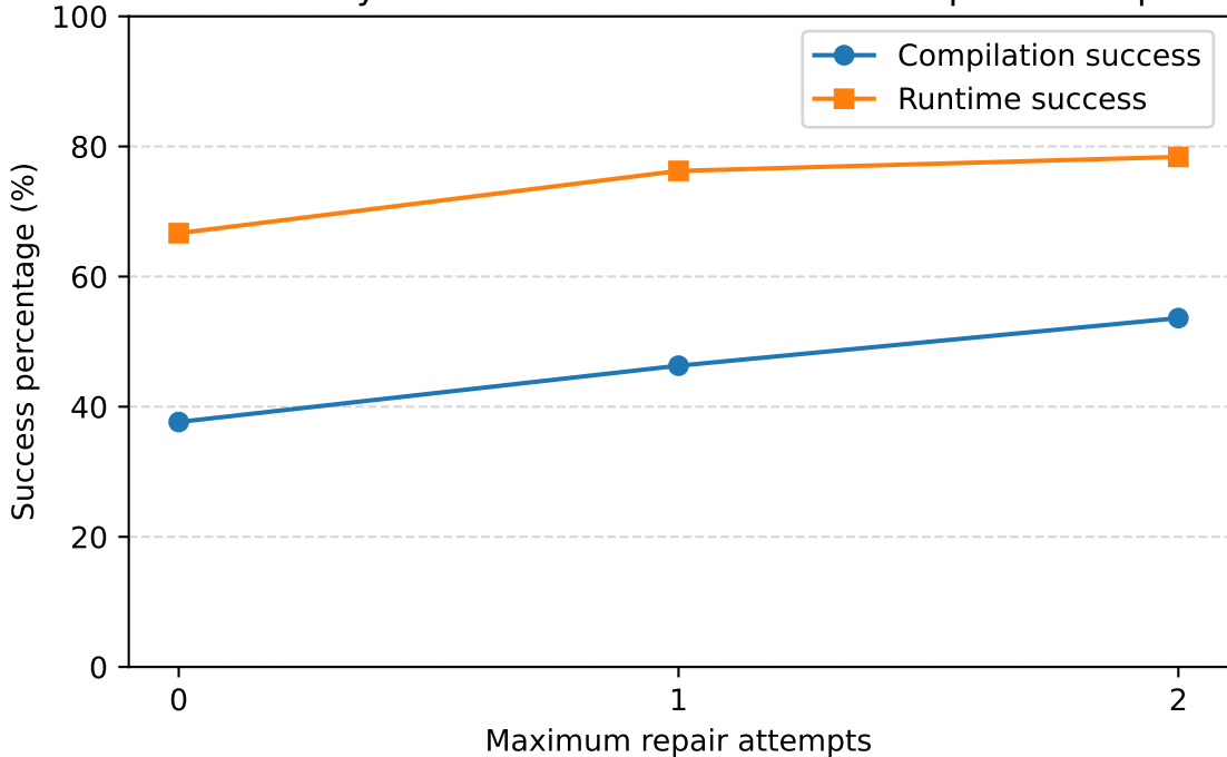
Test Validity Across Different Numbers of Repair Attempts
