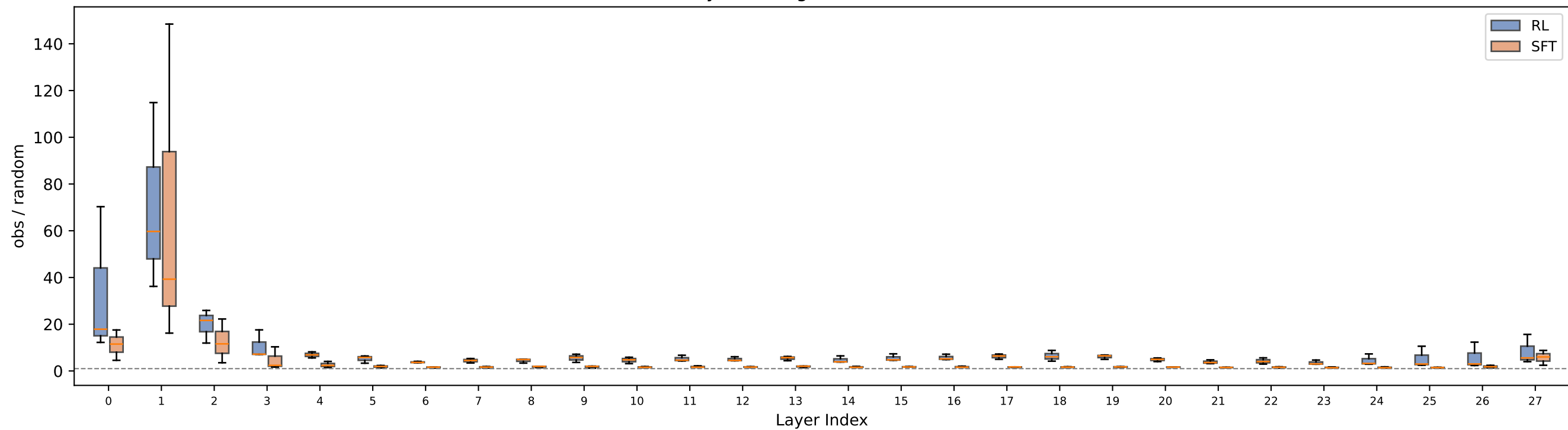
MLP Layers -- Alignment Ratio r(k=64)
