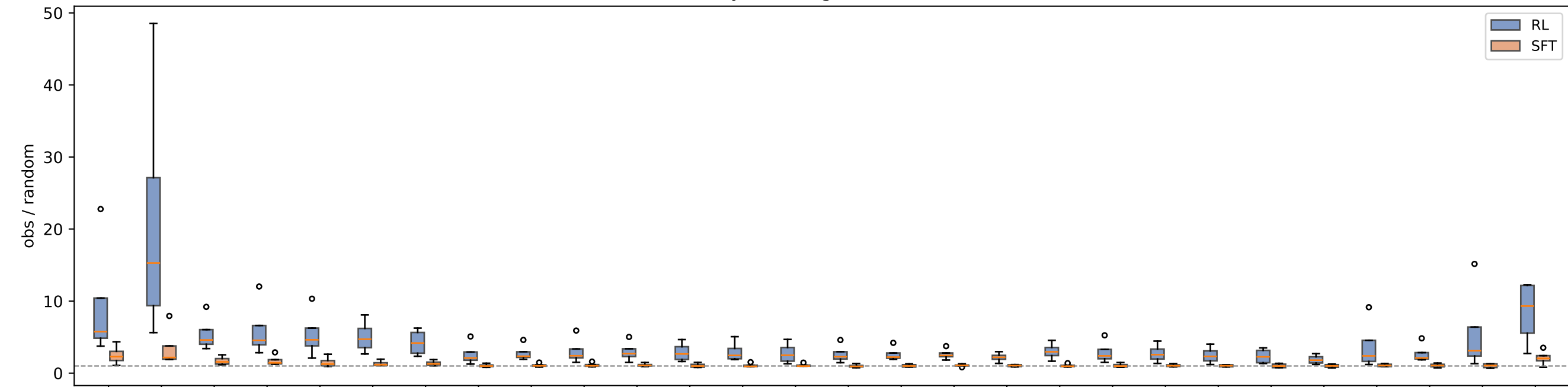
MLP Layers -- Alignment Ratio r(k=64)
