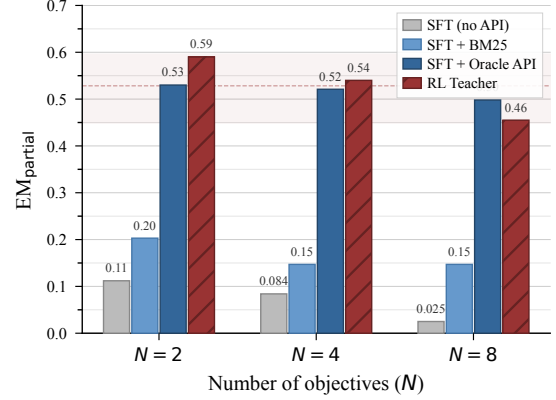
Figure 4: em\_partial under different retrieval conditions. Providing oracle retrieval results at inference time recovers the SFT student from near-zero to near-teacher performance across all N , while even a standard BM25 backend yields meaningful gains. The RL teacher (hatched) is shown for reference.
