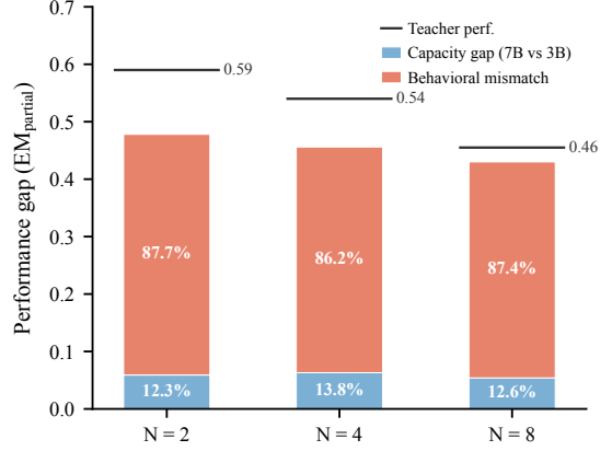
Figure 5: Teacher–student gap: two independent upper bounds, not a complementary partition. Capacity bound (\text{em}_{7B} - \text{em}_{3B}) / (\text{em}_{\text{teacher}} - \text{em}_{3B}) = 12.6\% at N = 8 . Retrieval-quality bound: oracle intervention recovers 110% of the teacher gap at N = 8 , exceeding 100% because the oracle replay isolates retrieval from search-strategy mismatch, while the teacher’s observed gap compounds both retrieval and search costs.
