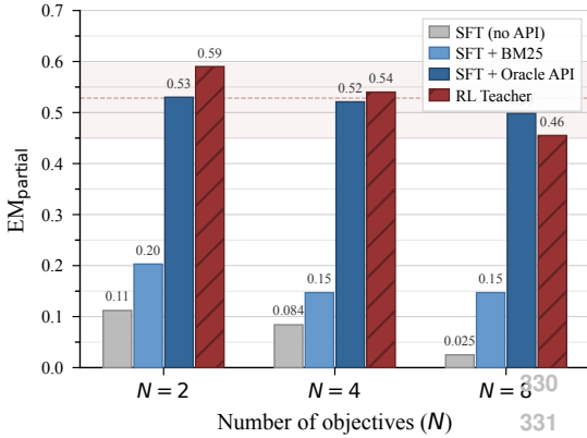
Figure 4: \text{em\_partial} under different retrieval conditions. Providing oracle retrieval results at inference time recovers the SFT student from near-zero to near-teacher performance across all N , while even a standard BM25 backend yields meaningful gains. The RL teacher (hatched) is shown for reference.
